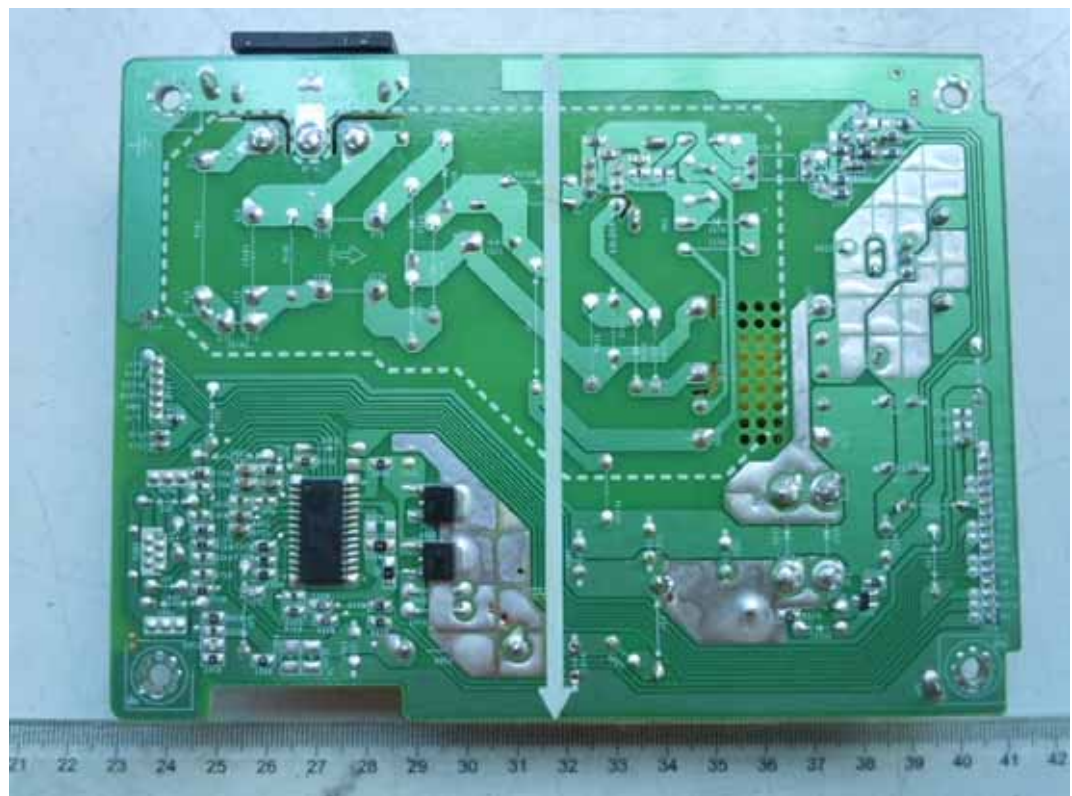
FIGURE 6 LCD MONITOR (M/N: E2541VX) POWER BOARD (SOLDERED SIDE)
