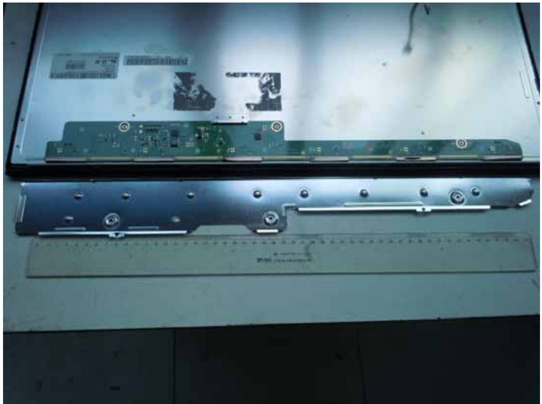
FIGURE 7 LCD MONITOR (M/N: E2541VX) LCD PANEL BOARD (COMPONENT SIDE)
