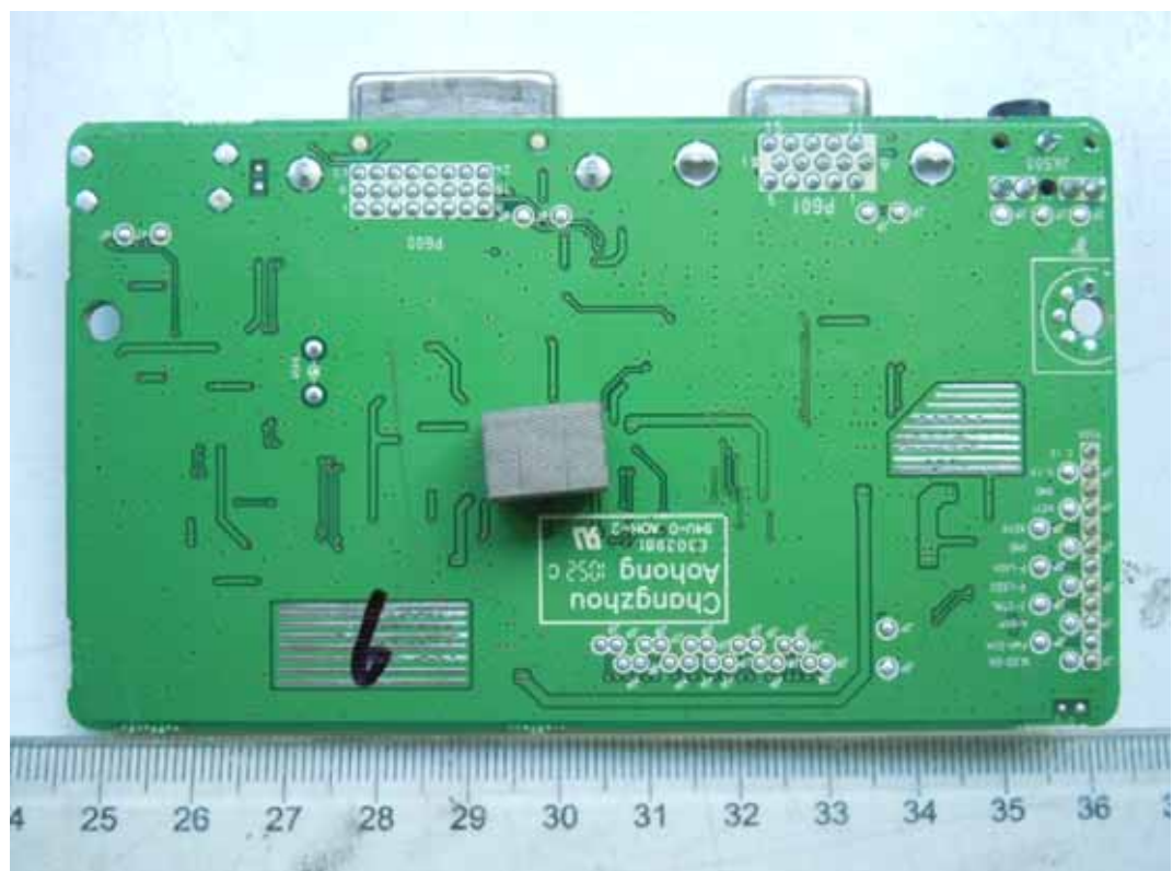
FIGURE 3 LCD MONITOR (M/N: E2541VX) MAIN BOARD (COMPONENT SIDE)
