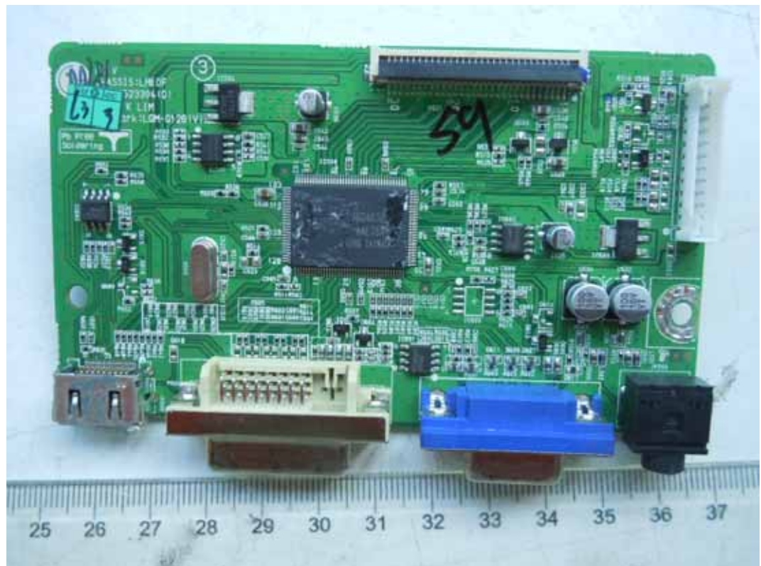
FIGURE 2 LCD MONITOR (M/N: E2541VX) MAIN BOARD (COMPONENT SIDE)
