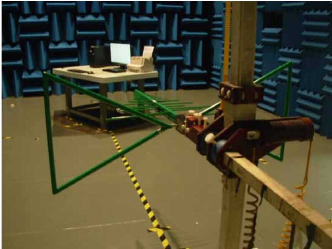
SETUP WITH MAXIMUM DETECTED EMISSION AT HORIZONTAL POLARIZATION (TEST MODE: DVI 640*480@60Hz)
