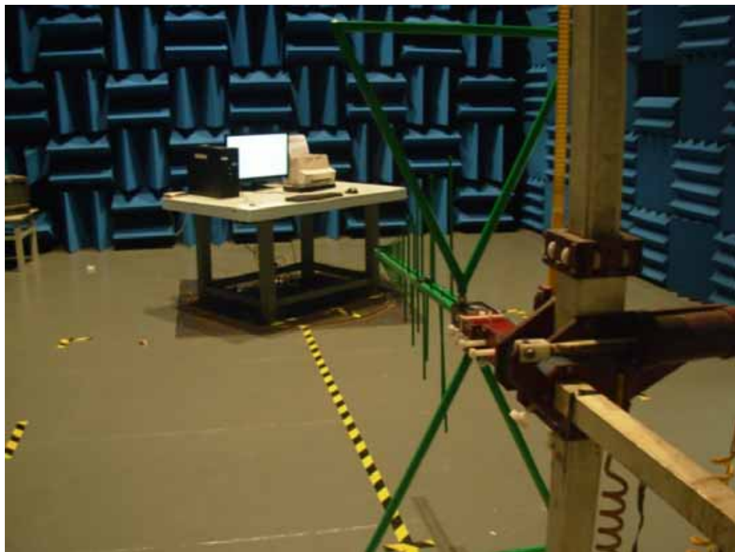
SETUP WITH MAXIMUM DETECTED EMISSION AT VERTICAL POLARIZATION (TEST MODE: DVI 640*480@60Hz)
