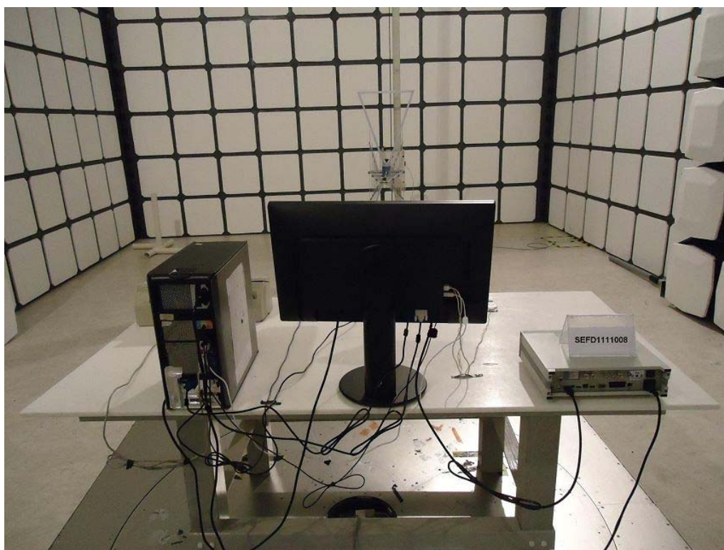
Back View of Radiated Emission Test (30MHz ~ 1000MHz)
