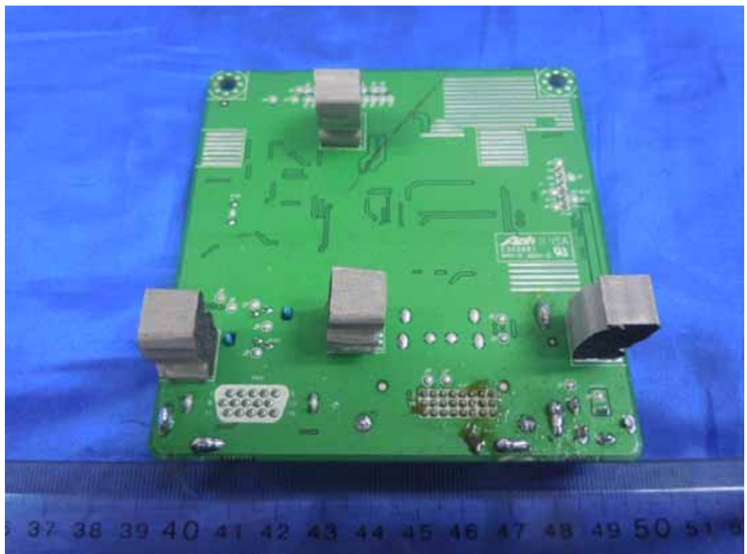
FIGURE 4 LCD MONITOR (M/N: E2742VA) MAIN BOARD (SOLDERED SIDE)
