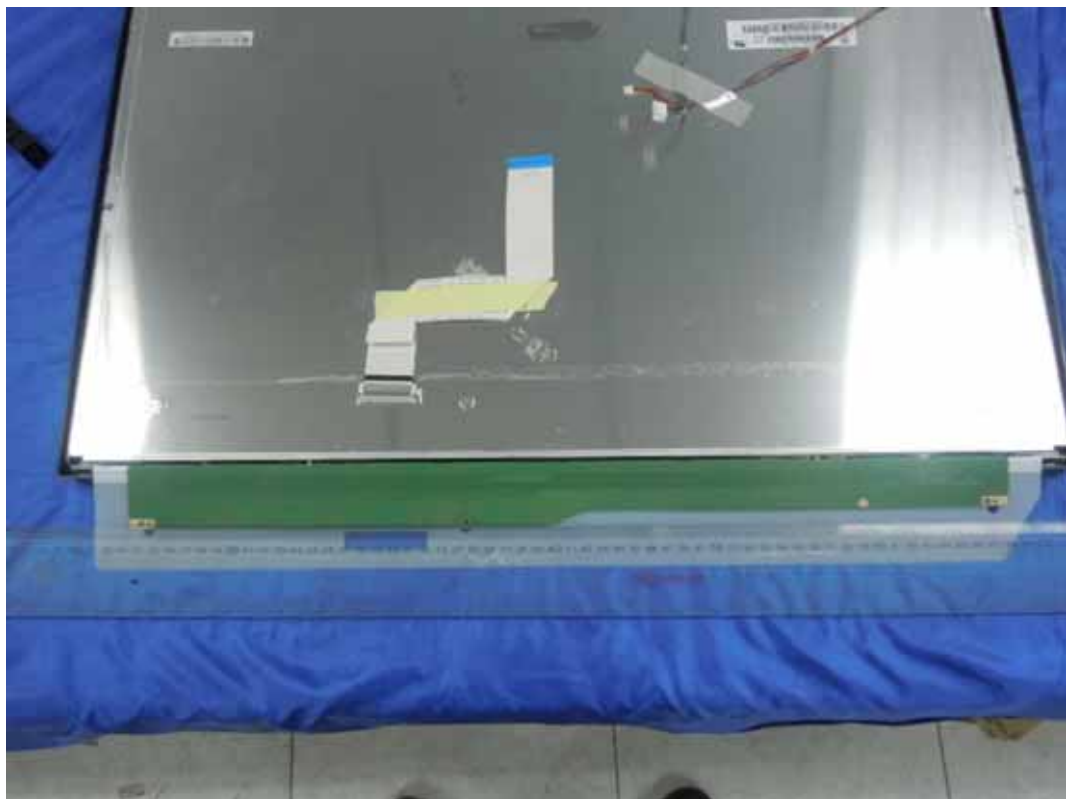
FIGURE 9 LCD MONITOR (M/N: E2742VA) LCD PANEL BOARD (SOLDERED SIDE)
