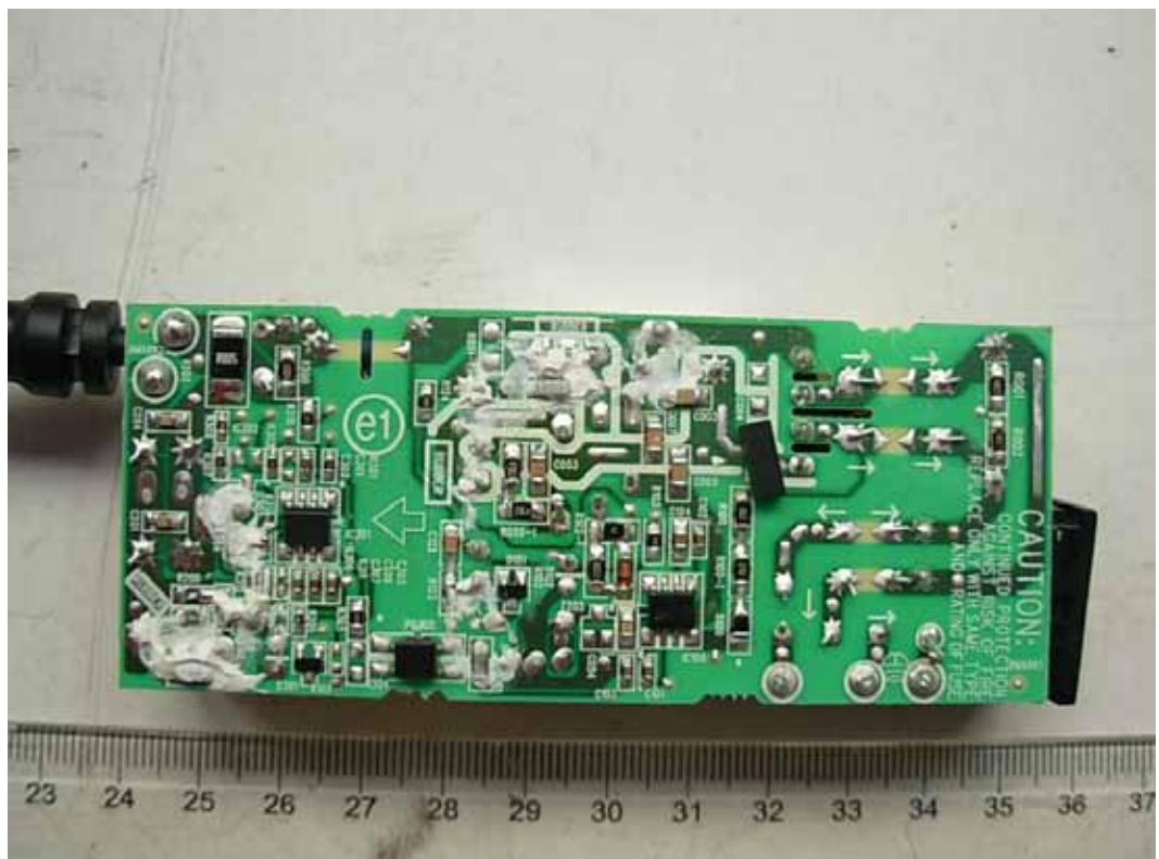
FIGURE 14 LCD MONITOR (M/N: E2750VV) ADAPTER (MAIN BOARD – SOLDERED SIDE)
