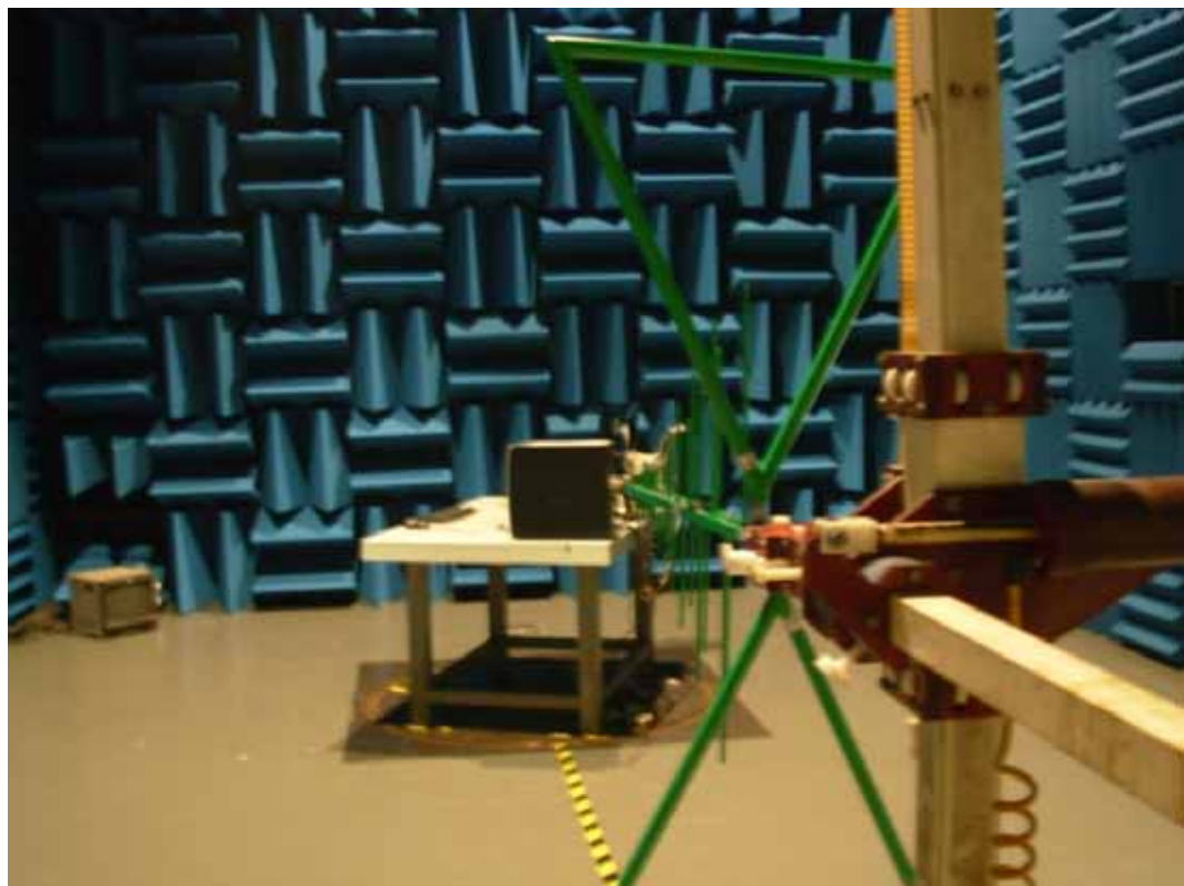
SETUP WITH MAXIMUM DETECTED EMISSION AT VERTICAL POLARIZATION (TEST MODE: HDMI 480P)
