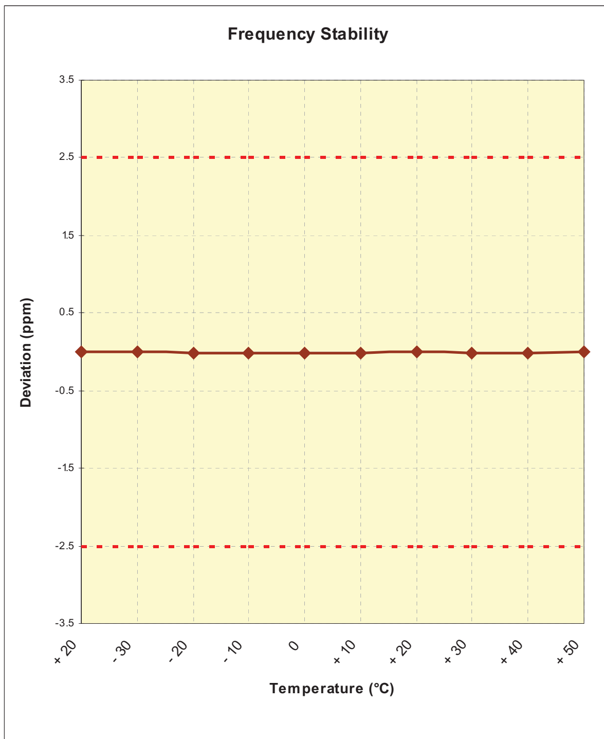
Figure 6-4. Frequency Stability Graph (PCS WCDMA Mode – Ch. 9400)
