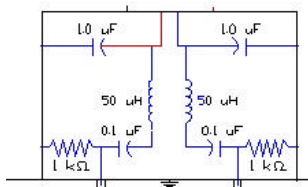
Fig. 3. LISN Schematic Diagram
