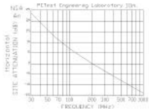
Fig. 5. NSA Theoretical Attenuation Curves (Horiz. Pol.)
