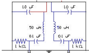
Fig. 3. LISN Schematic Diagram
