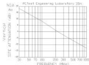
Fig. 6. NSA Theoretical Attenuation Curves (Vert. Pol.)
