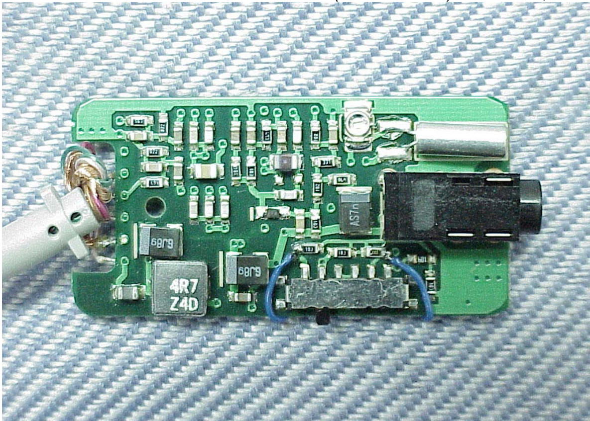
Photos 10 (FM Transmitter) Main Board, Back Side
