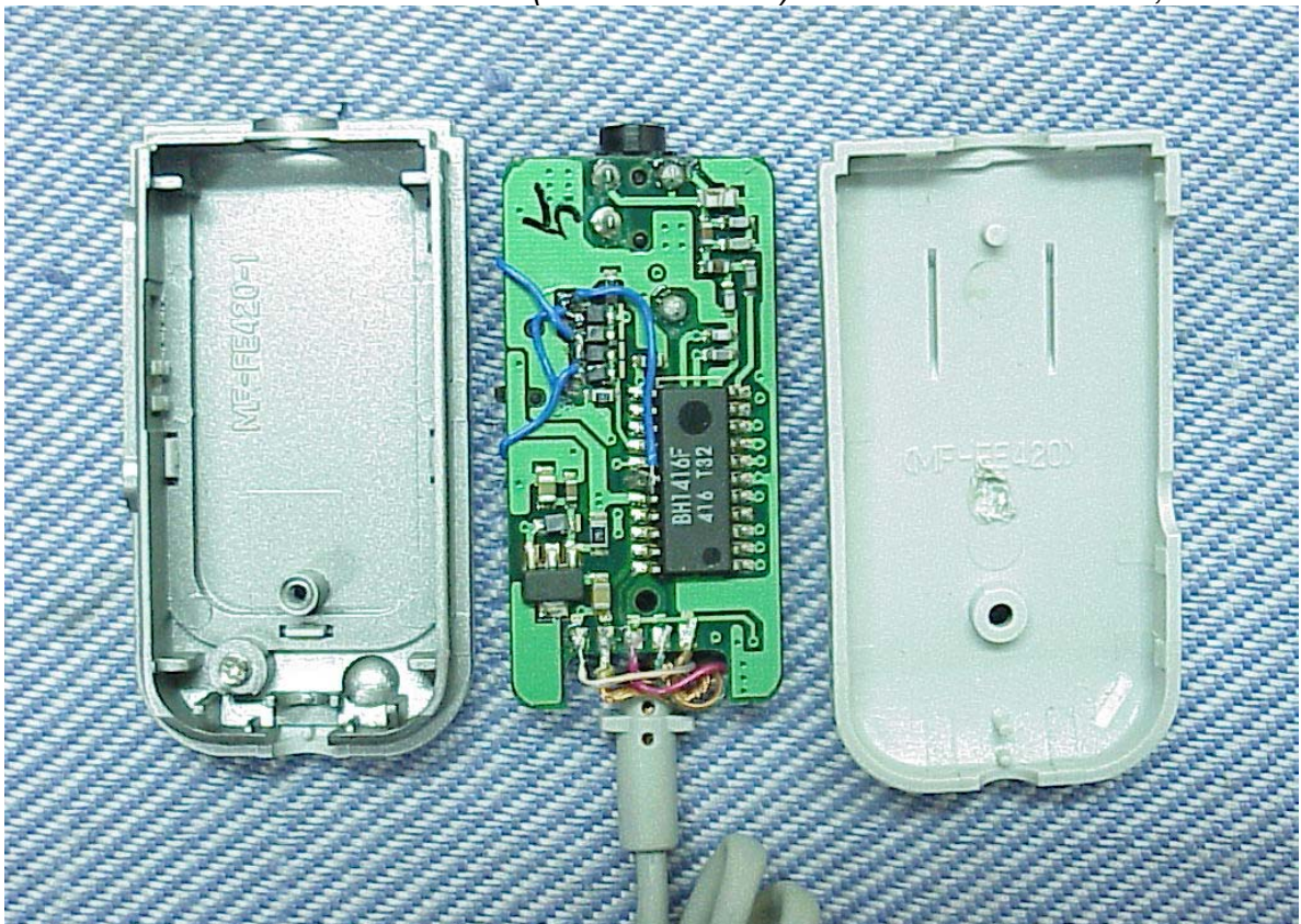
Photos 8 (FM Transmitter) Remove Case Covers, Internal View
