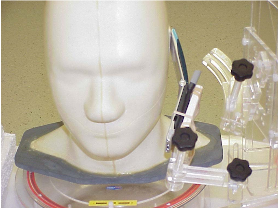
Photo 5. Left tilt
