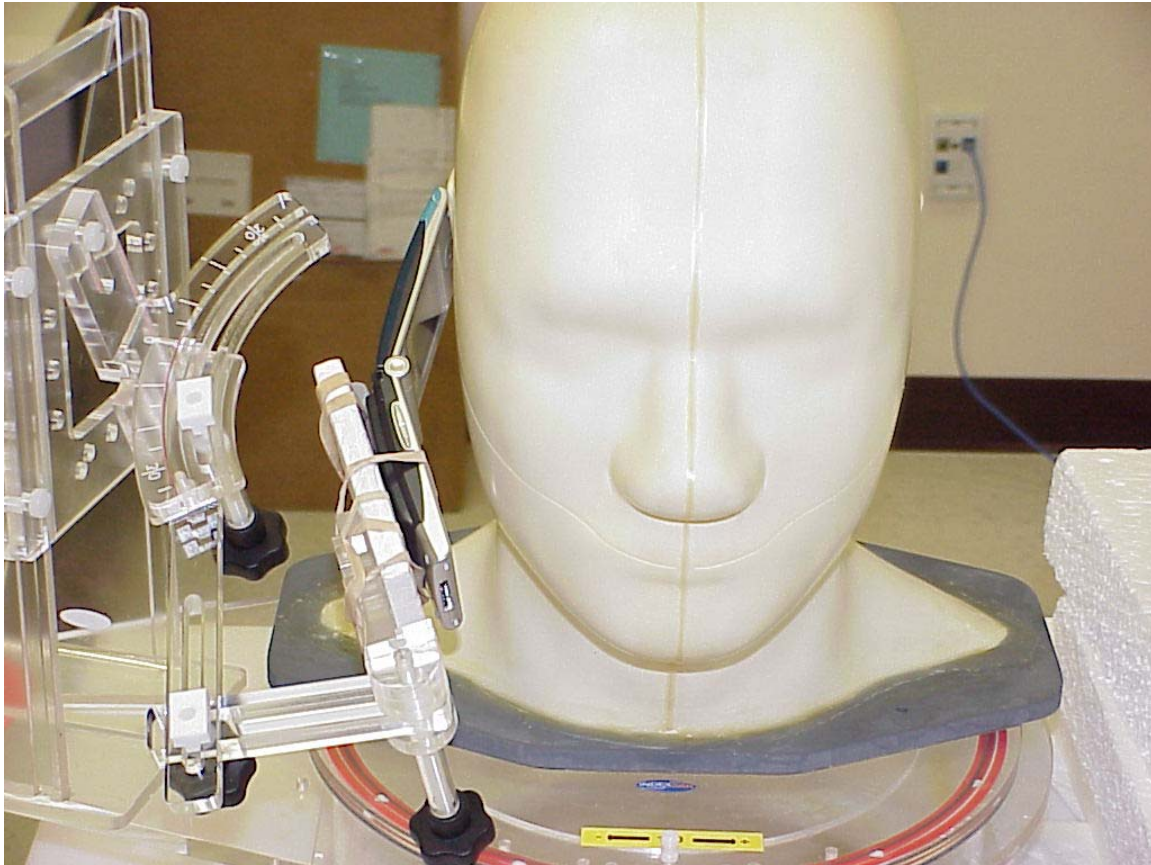
Photo 7. Right tilt
