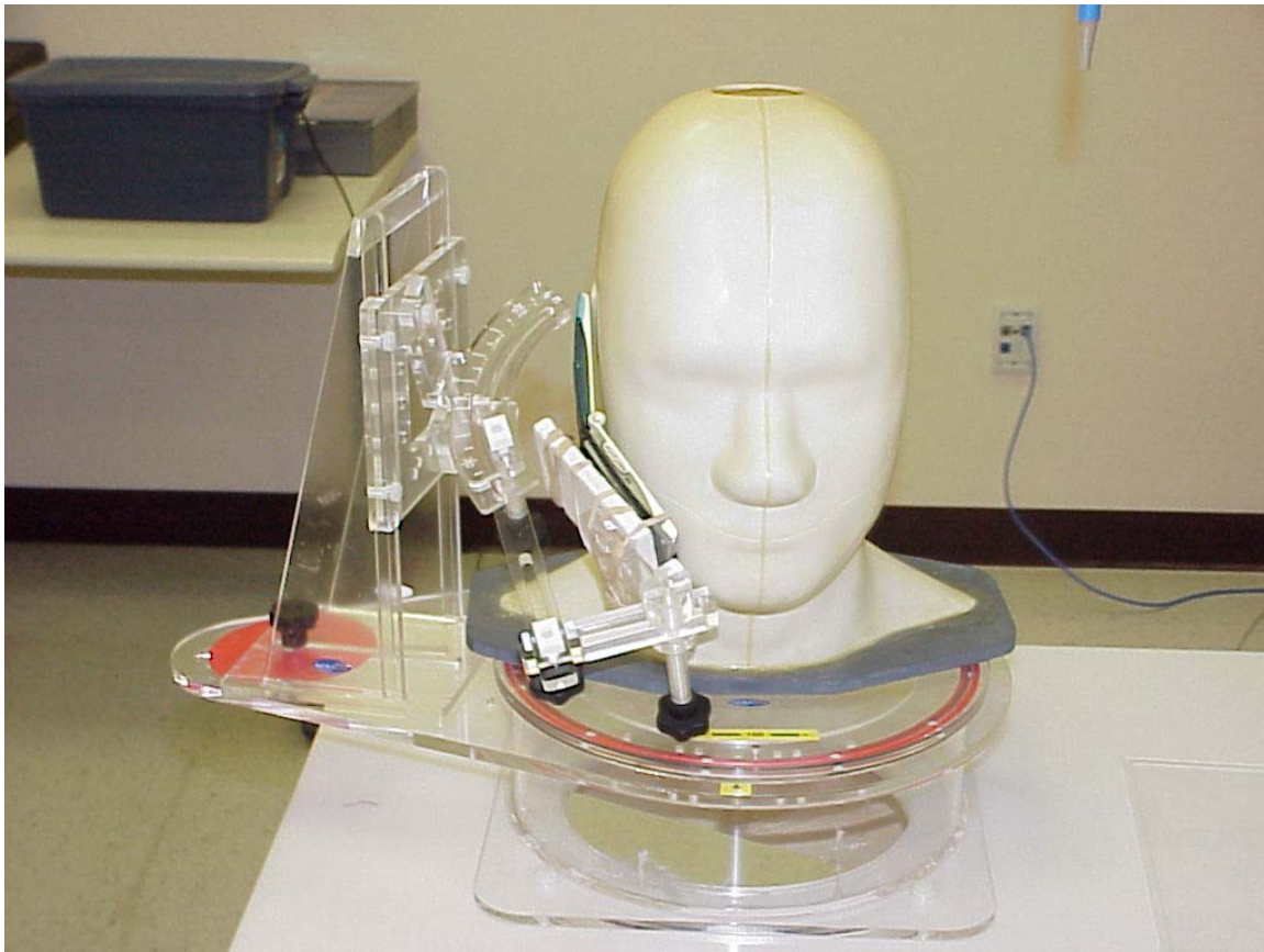
Photo 6. Right touch
