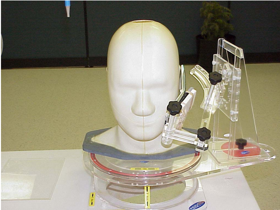
Photo 4. Left touch
