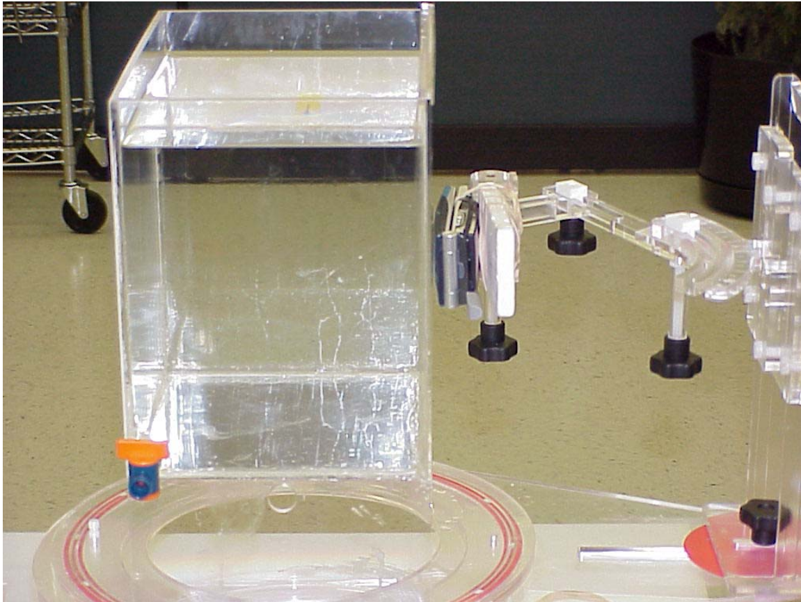
Photo 8. Body SAR
