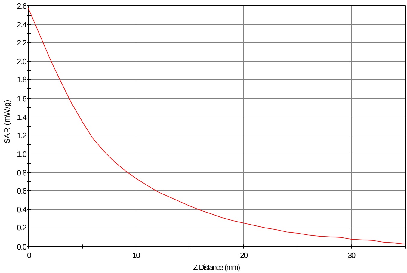
SAR - Z Axis at Hotspot x:76.0 y:15.0
