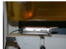
Figure A.5 Body SAR Test Setup -- w/o Belt Clip --
