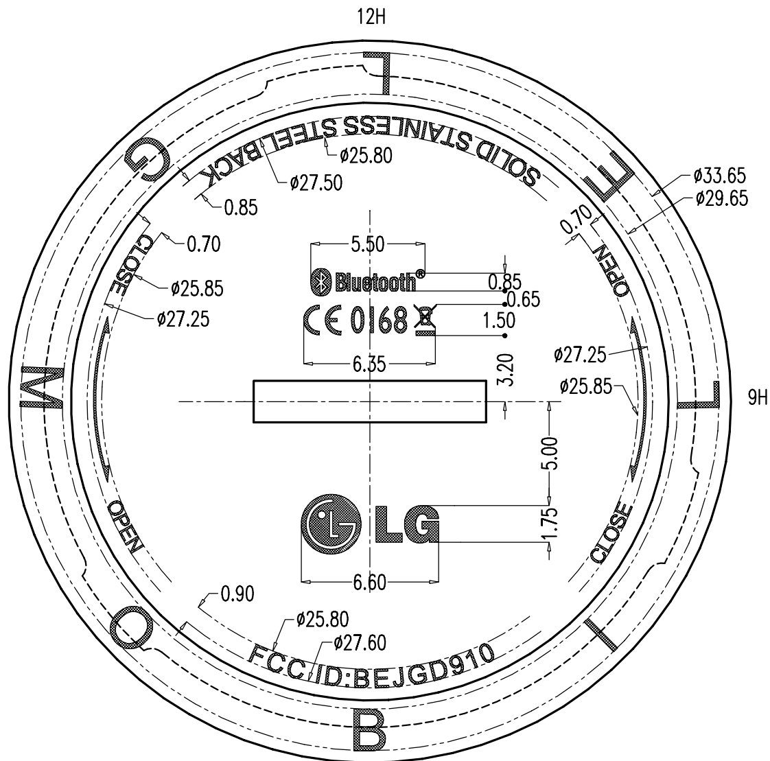
BACK OUTSIDE MARKINGS SCALE 4 : 1 DEEP ACID ETCHING VERSION 2
