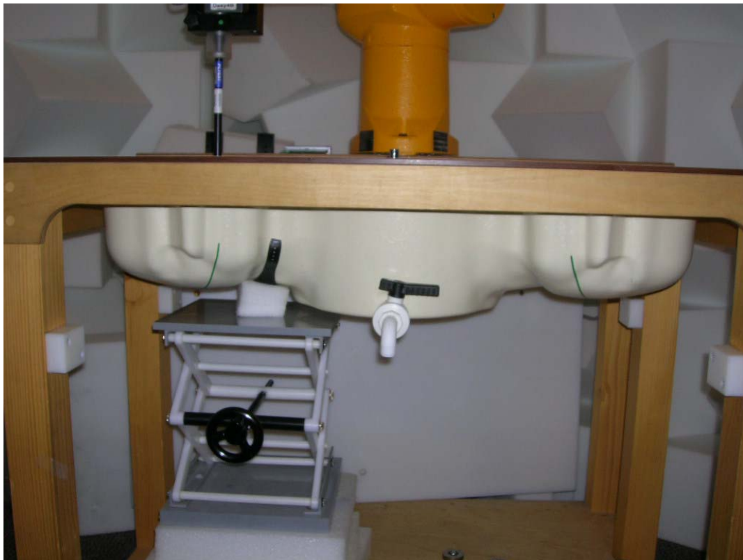
Figure 2 Wrist SAR Setup
