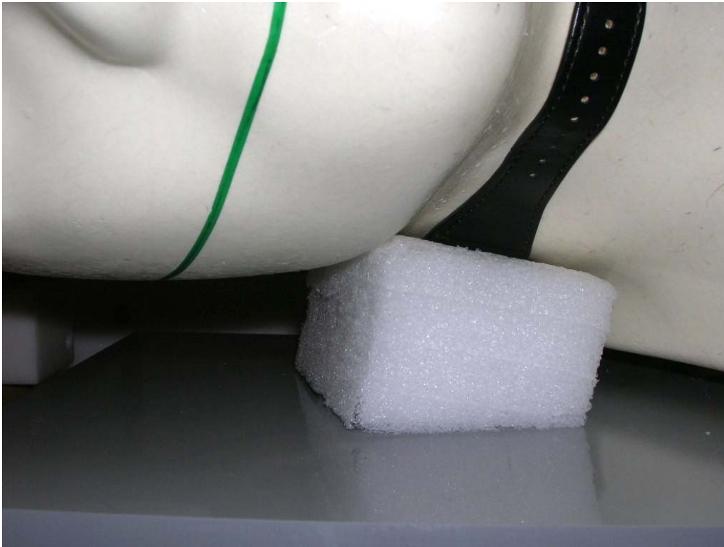
Figure 3 Wrist SAR Setup (close up), 0 cm spacing
