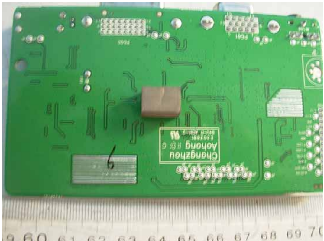
FIGURE 12 LCD MONITOR (M/N: IPS225VX) DEBUG #2
