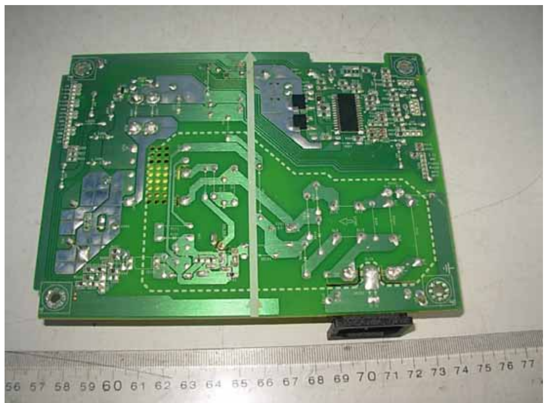
FIGURE 6 LCD MONITOR (M/N: IPS225VX) POWER BOARD (SOLDERED SIDE)
