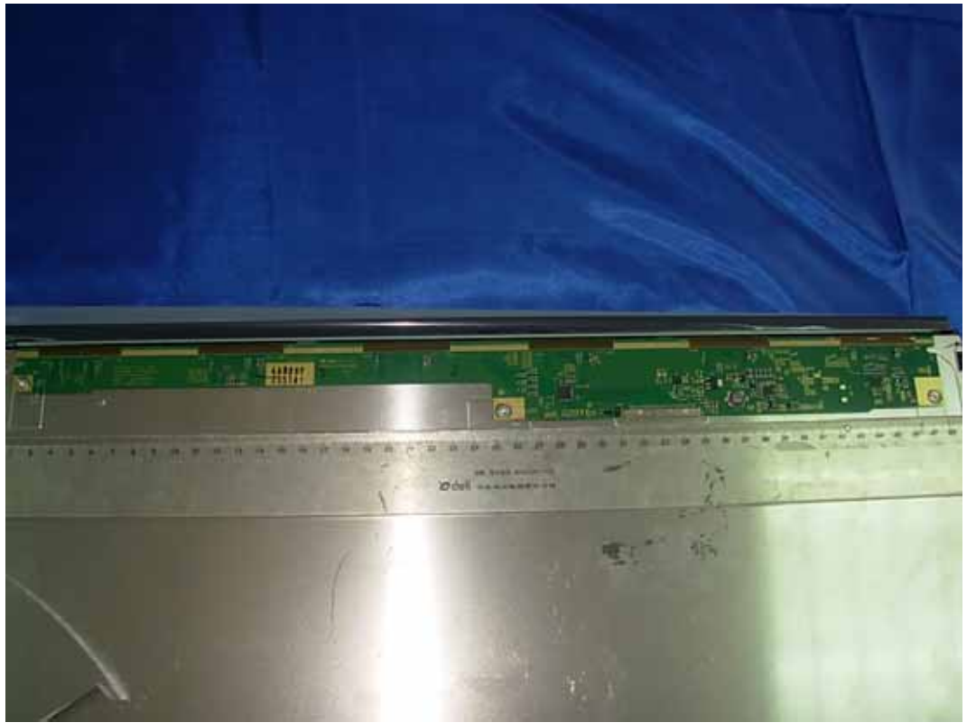
FIGURE 6 LCD MONITOR (M/N: IPS226TX) DISPLAY BOARD (COMPONENT SIDE)
