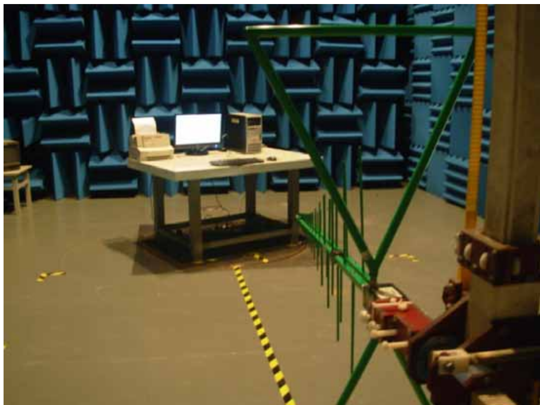
SETUP WITH MAXIMUM DETECTED EMISSION AT VERTICAL POLARIZATION (TEST MODE: DVI 640*480@60Hz, ADAPTER #1)
