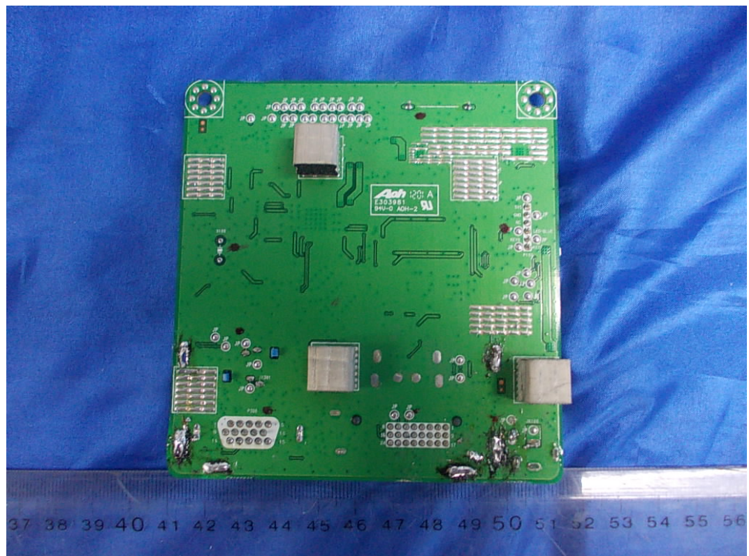
FIGURE 4 LCD MONITOR (M/N: IPS234VA) MAIN BOARD (SOLDERED SIDE)
