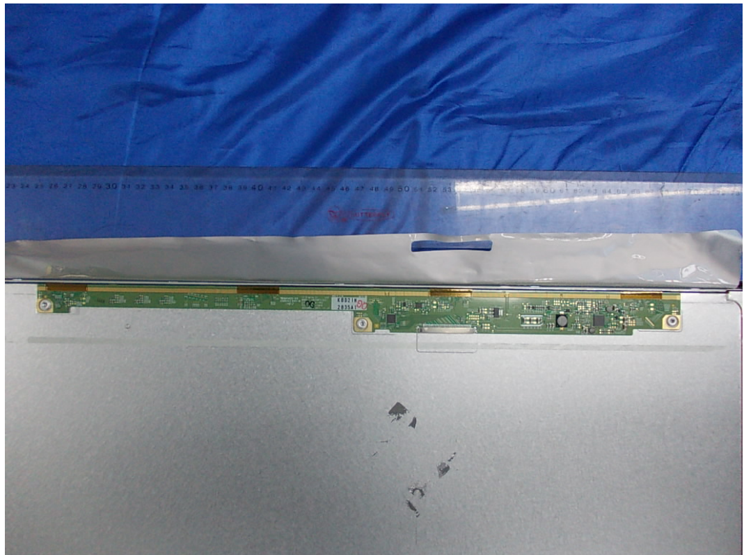
FIGURE 8 LCD MONITOR (M/N: IPS234VA) LCD PANEL BOARD (COMPONENT SIDE)
