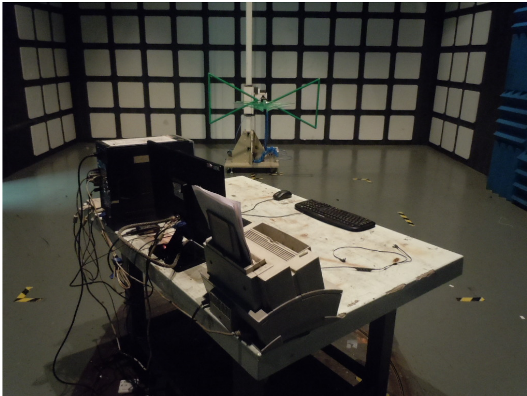
SETUP WITH MAXIMUM DETECTED EMISSION AT HORIZONTAL POLARIZATION (TEST MODE: DVI 1920*1080@60Hz ADAPTER #1)
