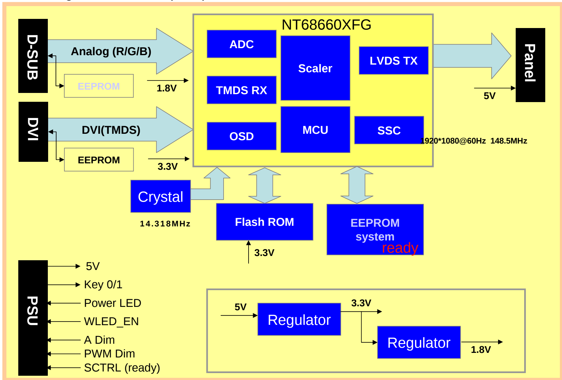
Block diagram for IPS5T (NVT)
