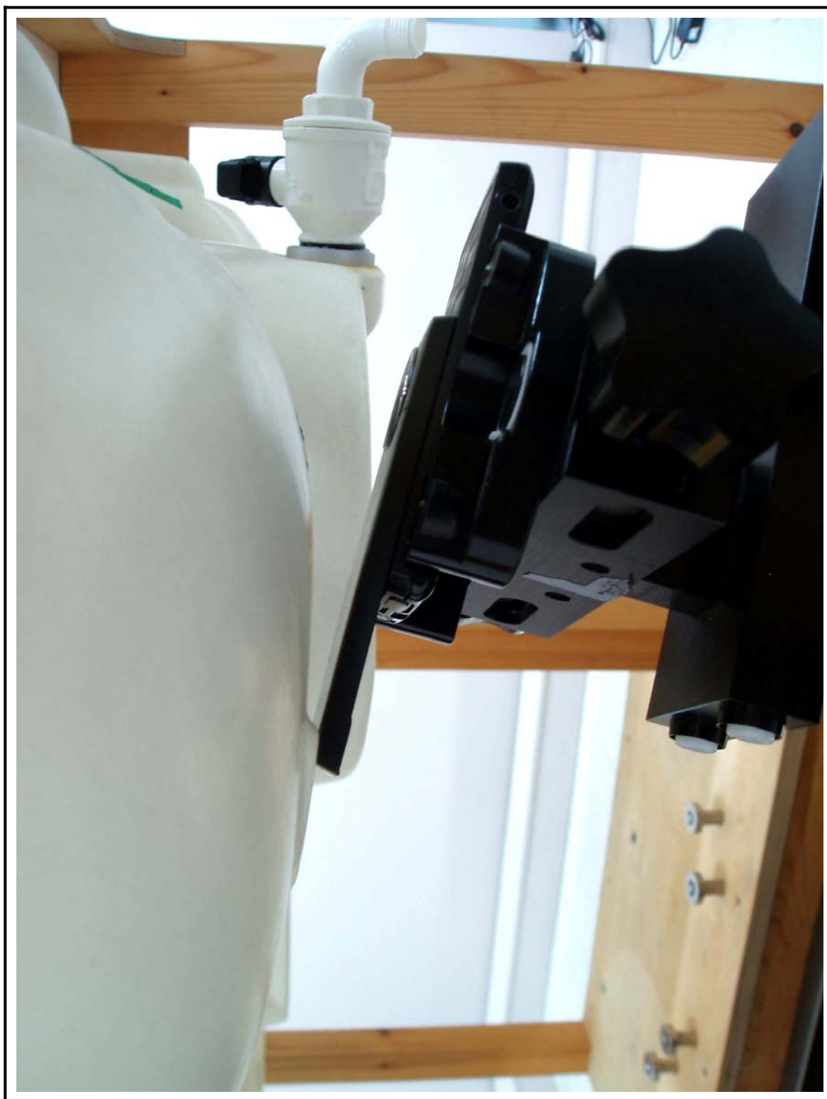
Figure 4 Right Head SAR Test Setup - Ear Tilt Position
