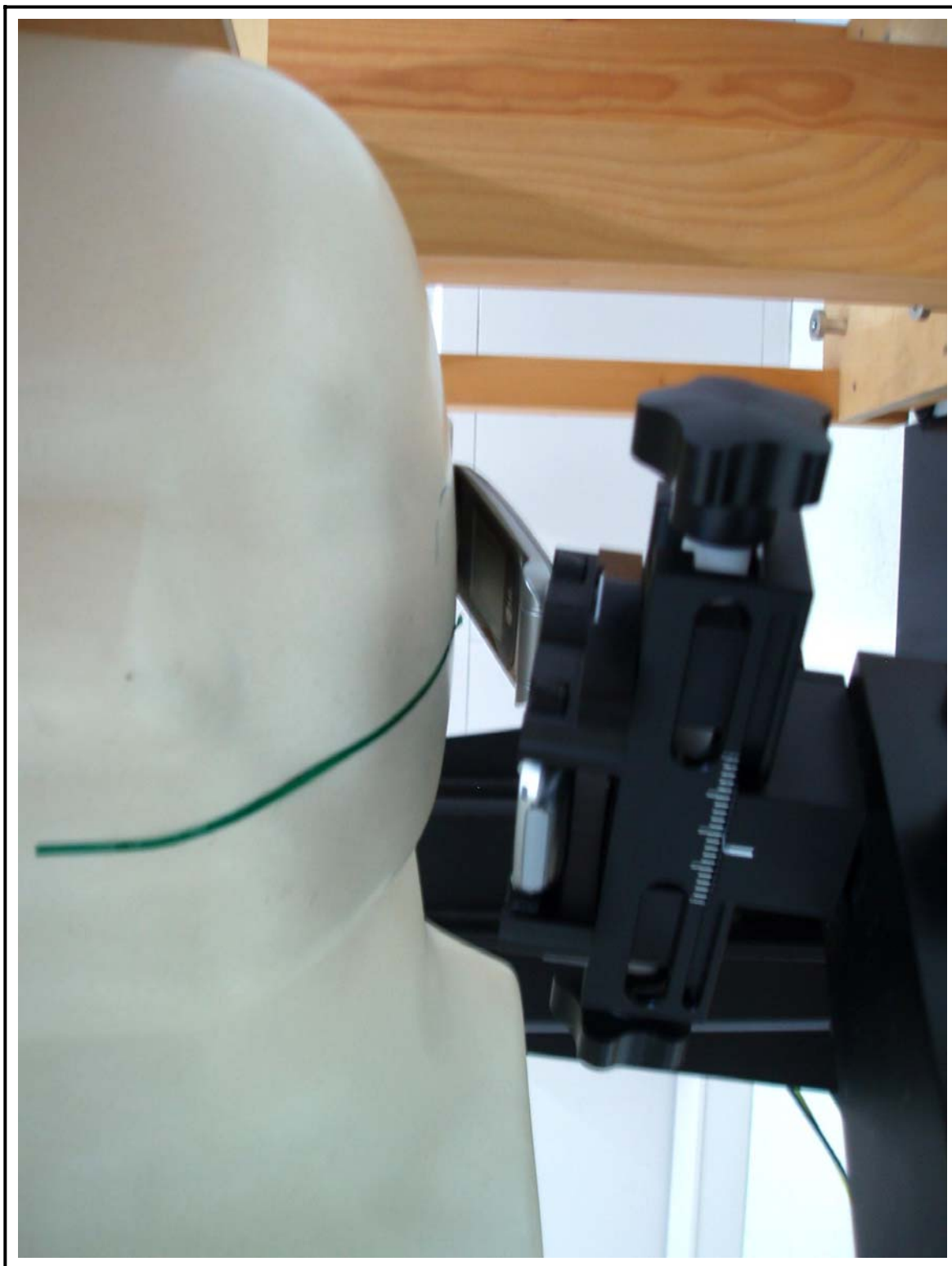
Figure 11 Left Head SAR Test Setup – Ear Tilt Position
