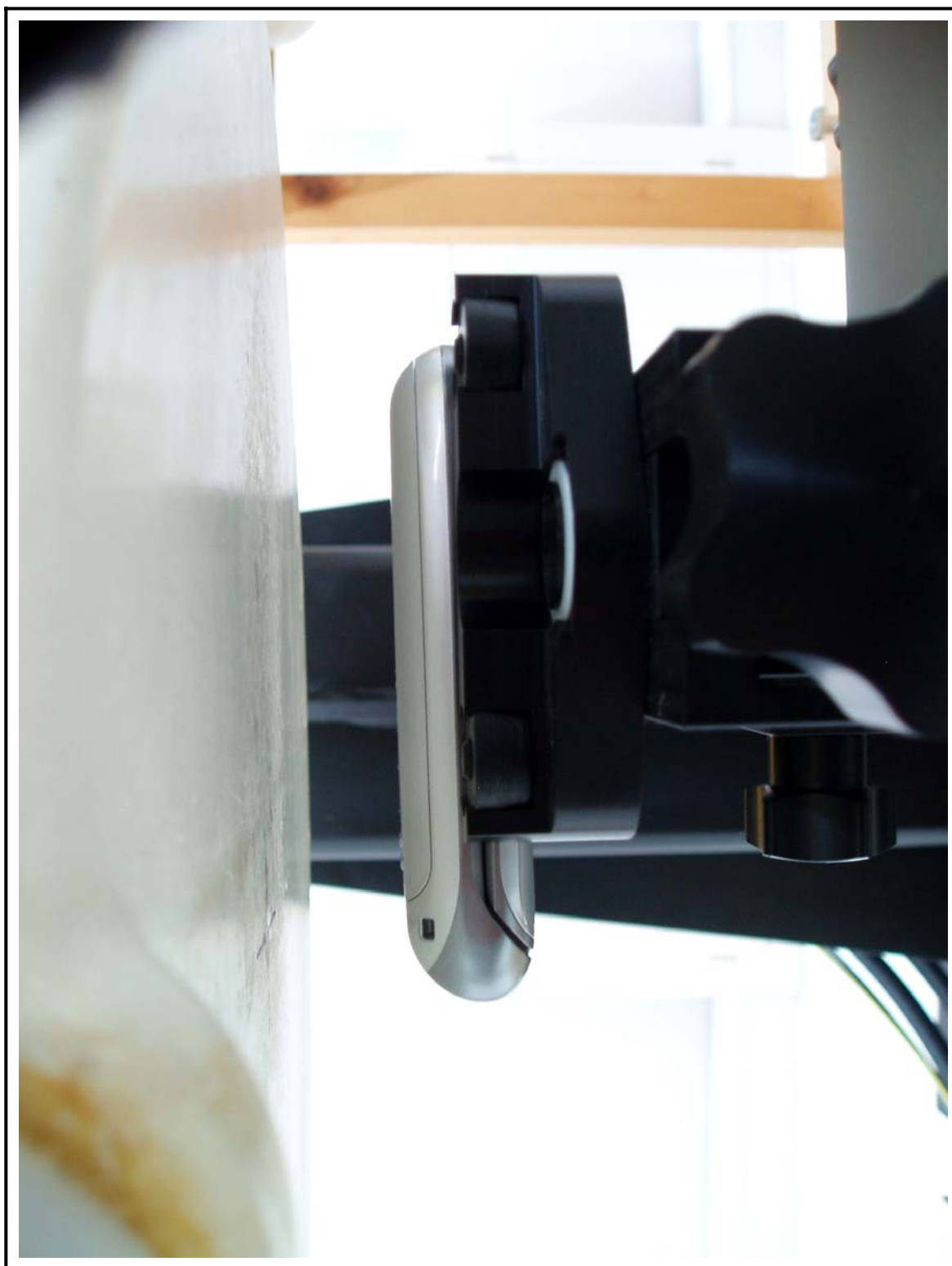
Figure 7 Body SAR Test Setup – w/o Holster
