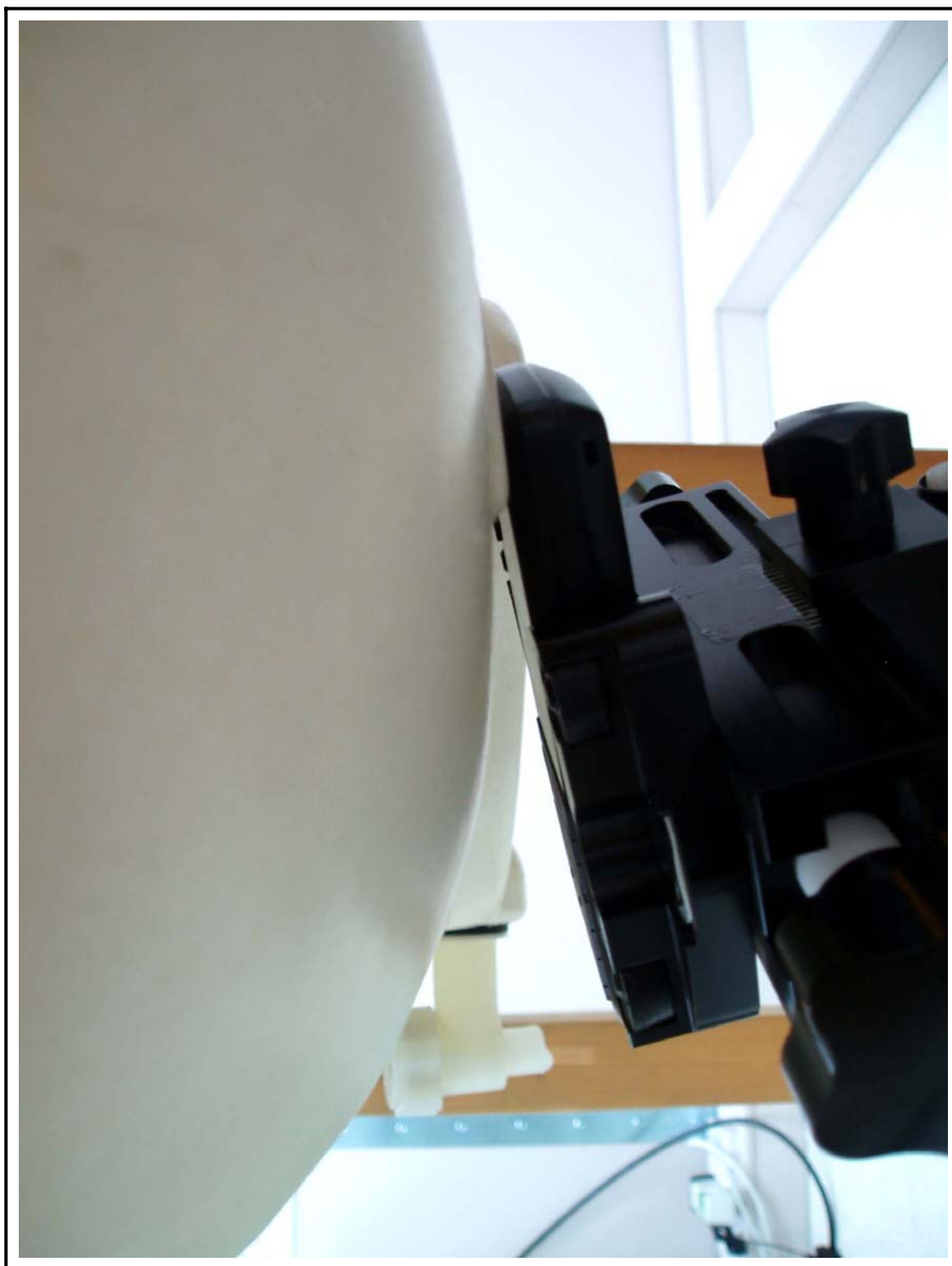
Figure 12 Left Head SAR Test Setup – Ear Tilt Position
