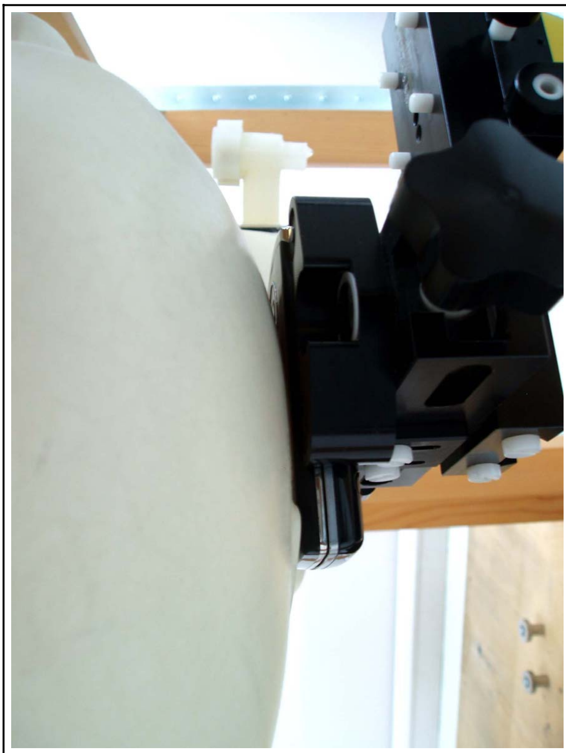
Figure 3 Right Head SAR Test Setup - Cheek Touch Position
