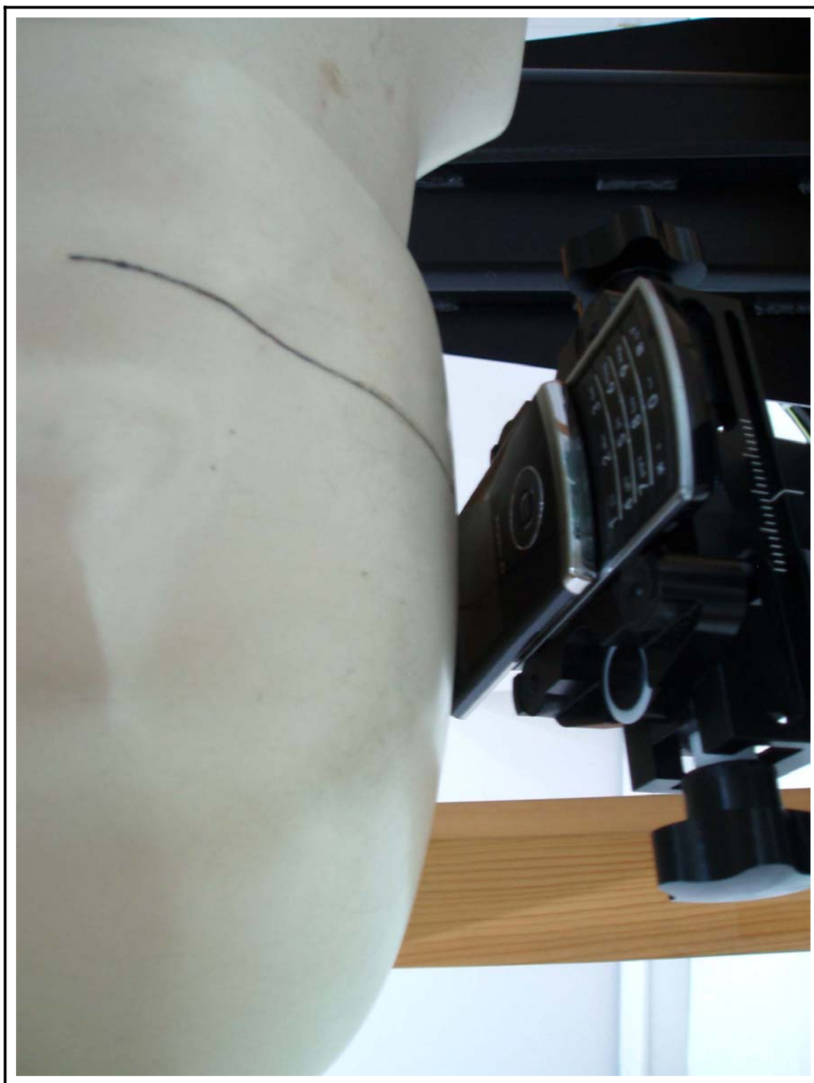
Figure 11 Right Head SAR Test Setup – Ear Tilt Position
