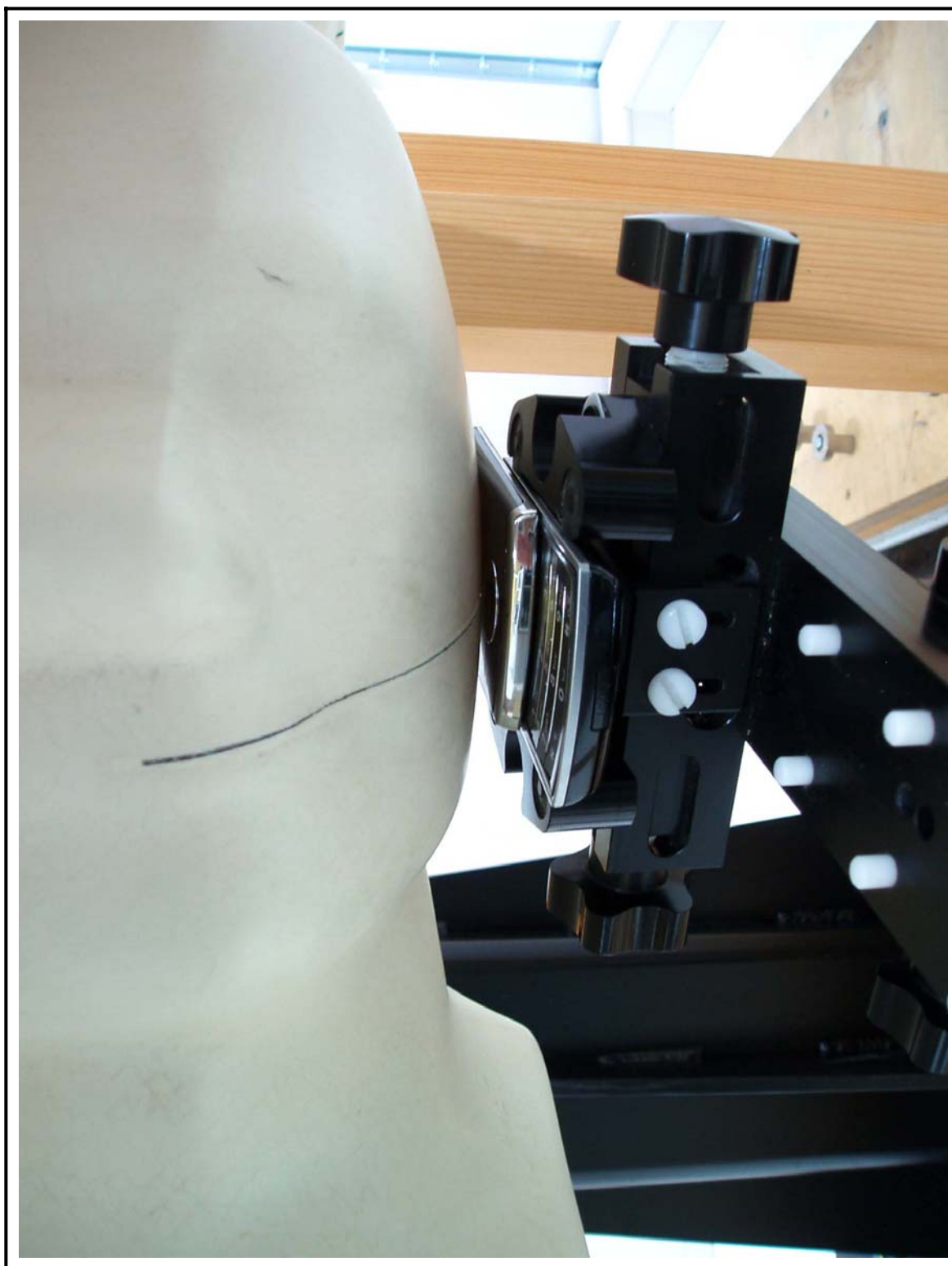
Figure 17 Left Head SAR Test Setup – Cheek Touch Position
