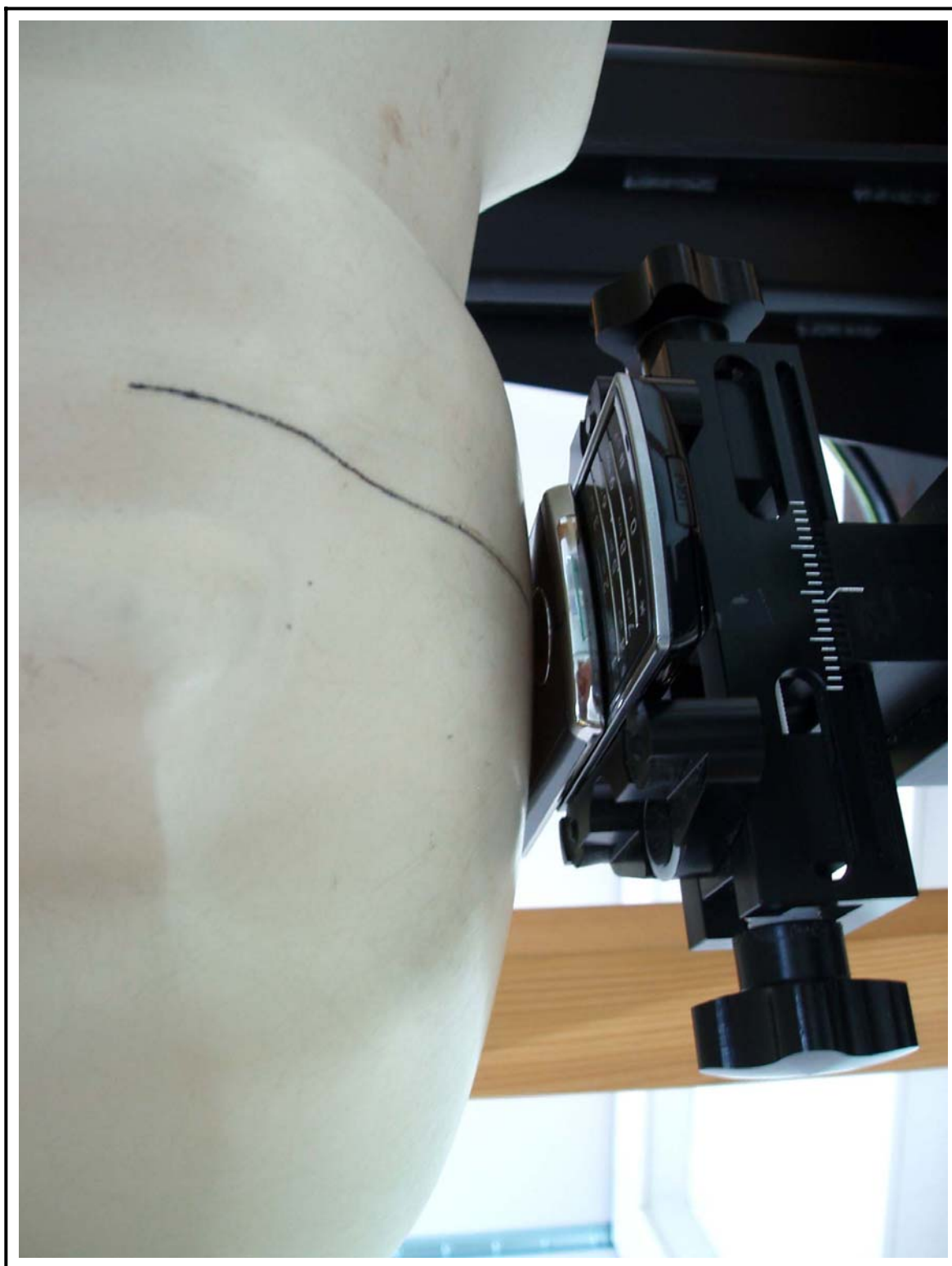
Figure 5 Right Head SAR Test Setup – Cheek Touch Position
