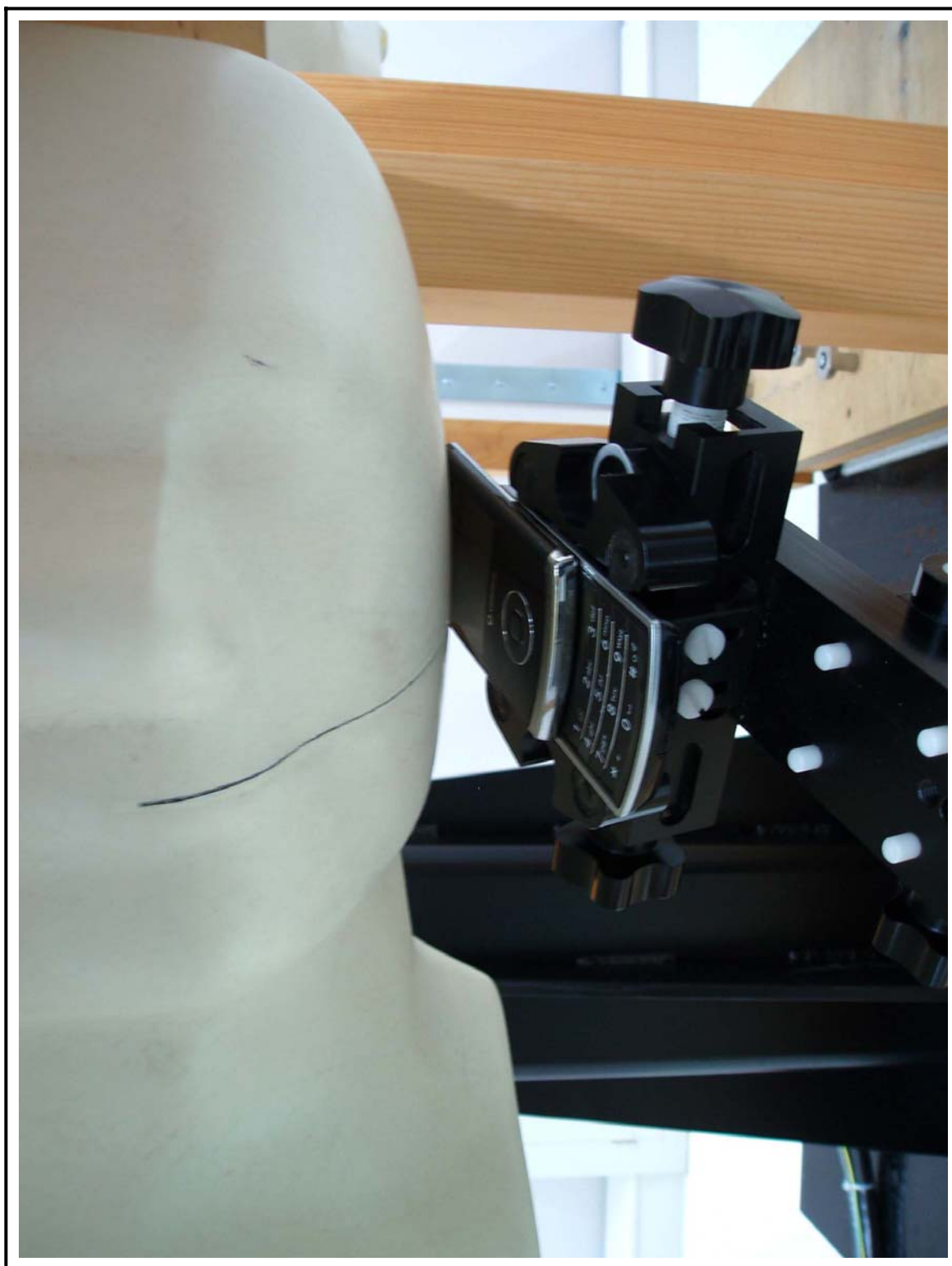
Figure 23 Left Head SAR Test Setup – Ear Tilt Position
