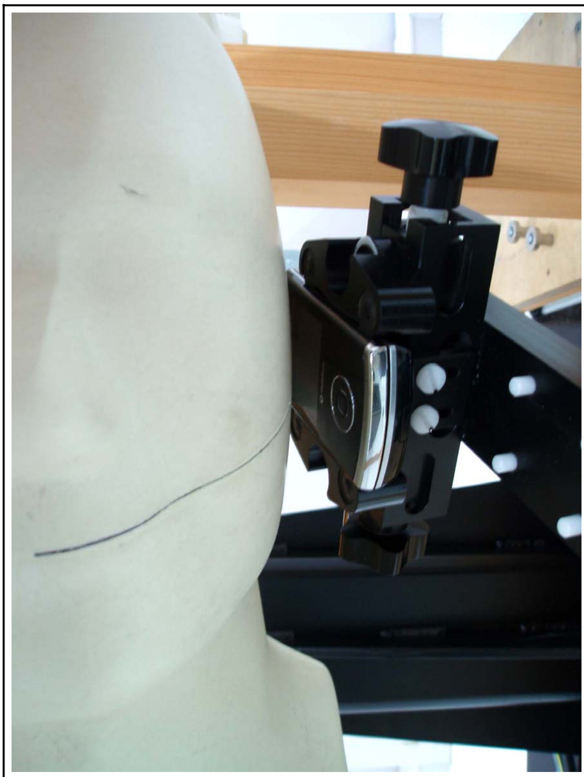
Figure 21 Left Head SAR Test Setup – Ear Tilt Position
