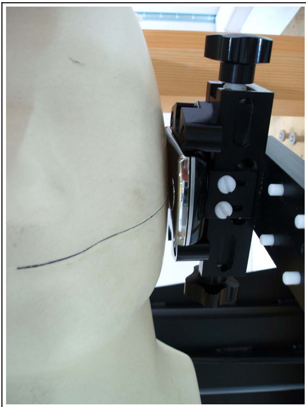
Figure 14 Left Head SAR Test Setup – Cheek Touch Position
