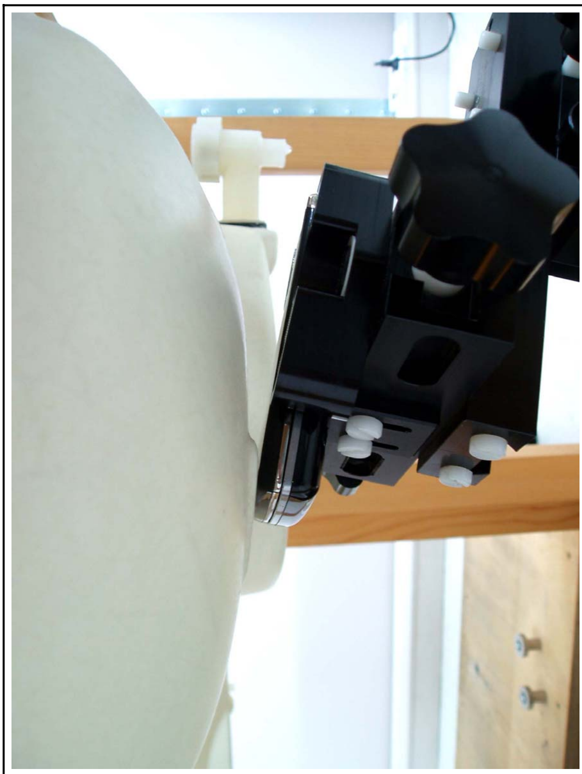
Figure 9 Right Head SAR Test Setup – Ear Tilt Position
