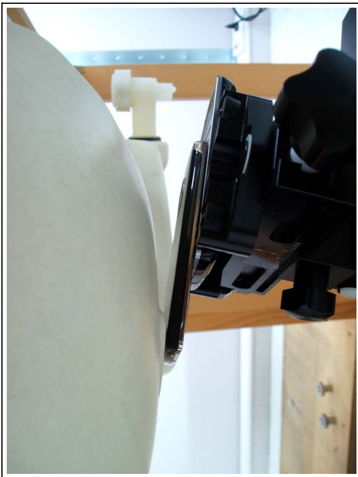
Figure 12 Right Head SAR Test Setup – Ear Tilt Position
