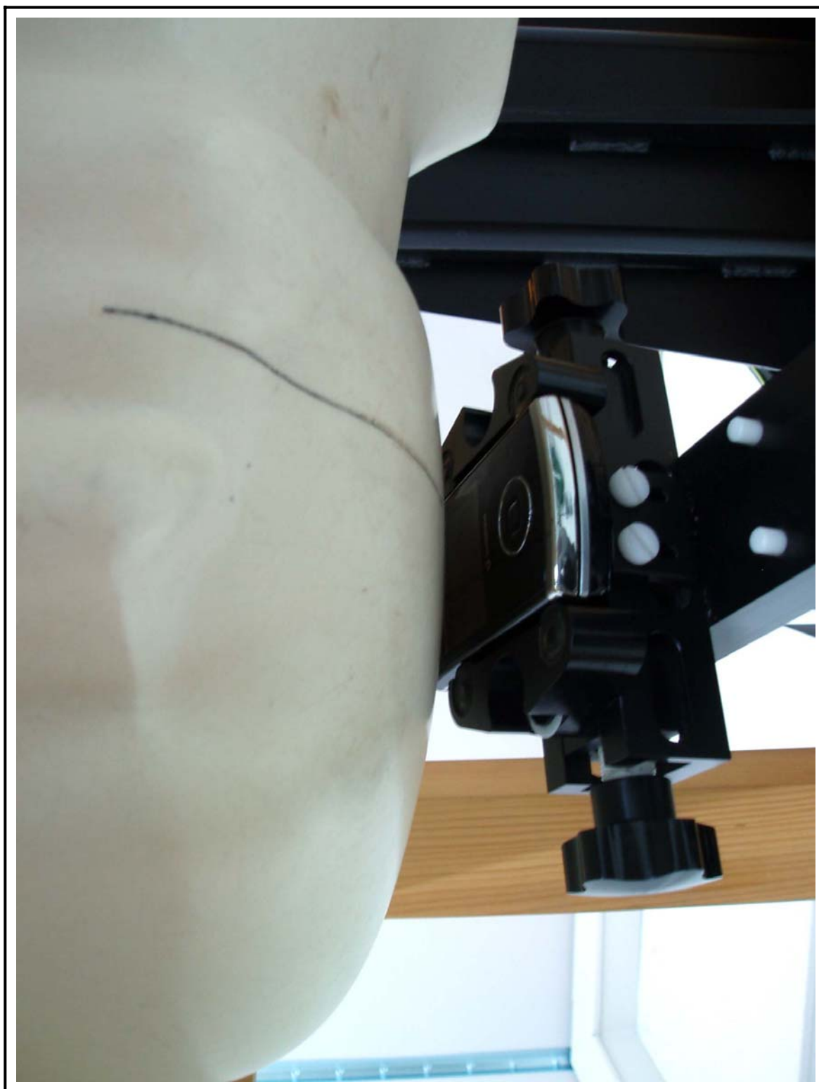
Figure 8 Right Head SAR Test Setup – Ear Tilt Position
