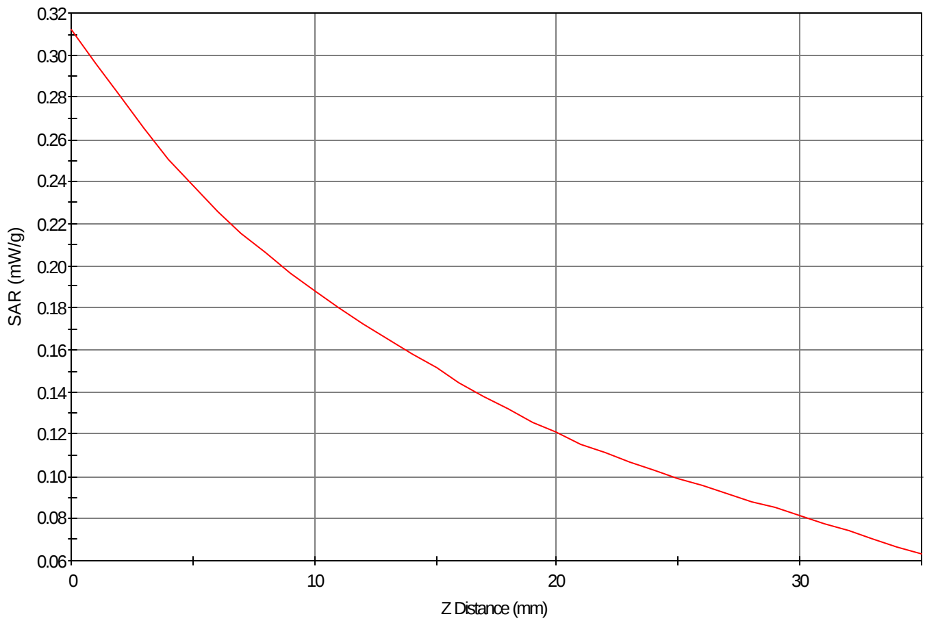
SAR - Z Axis at Hotspot x:64.0 y:9.0
