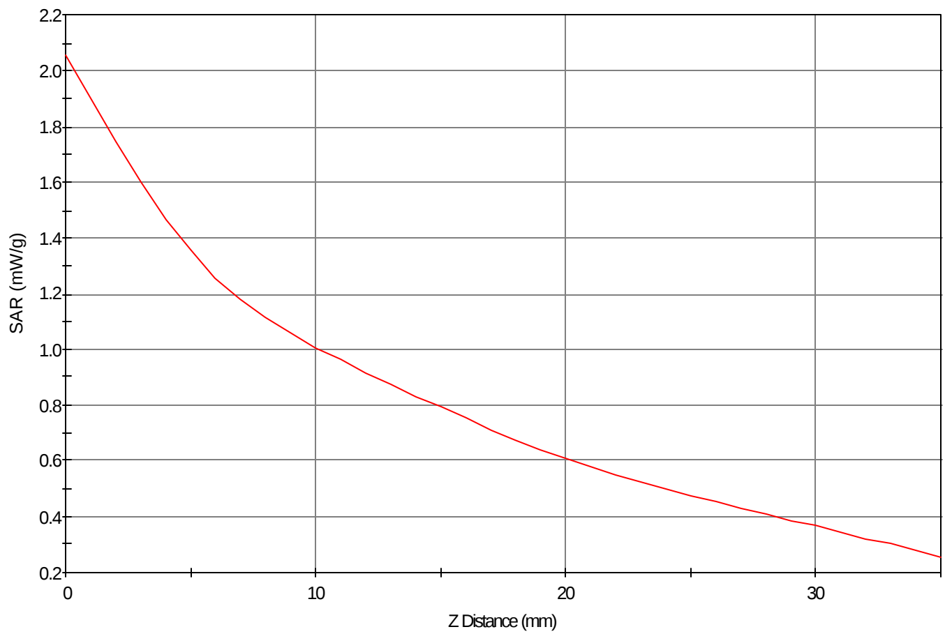
SAR - Z Axis at Hotspot x:77.0 y:20.0
