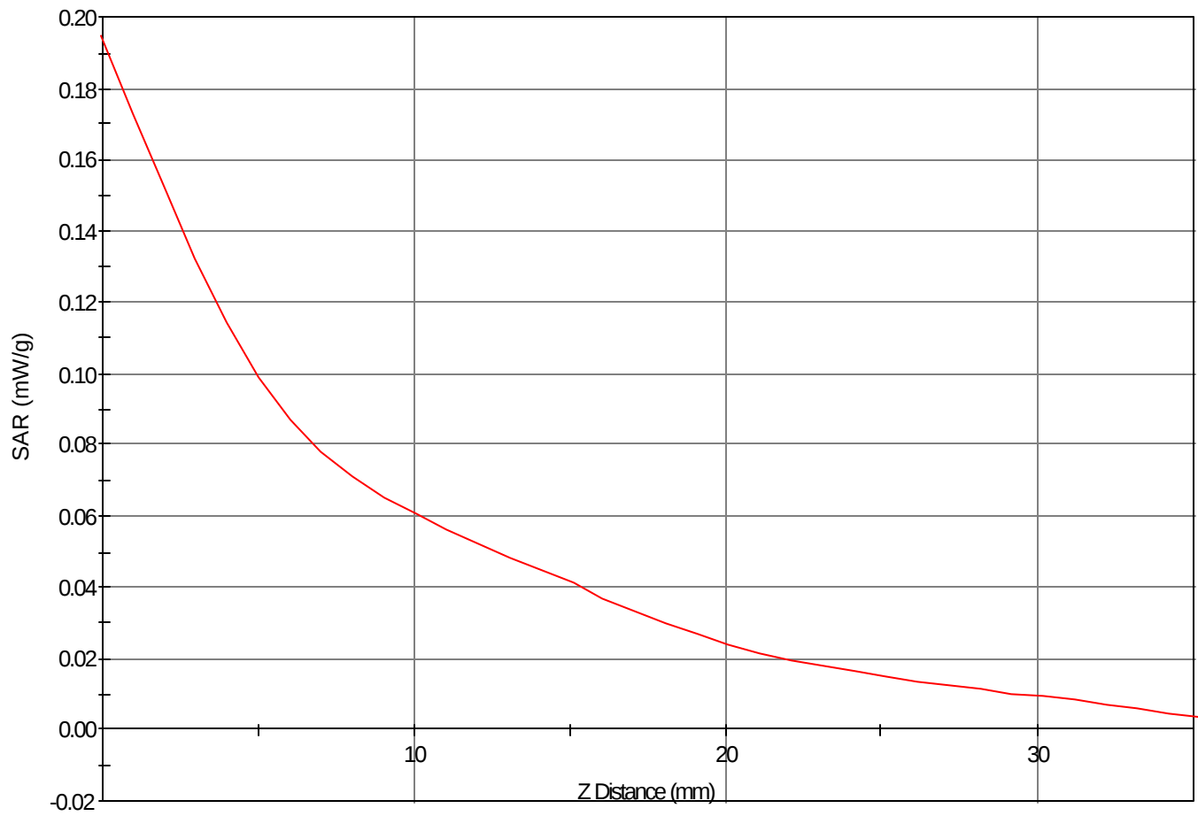
SAR - Z Axis at Hotspot x:8.0 y:-7.0
