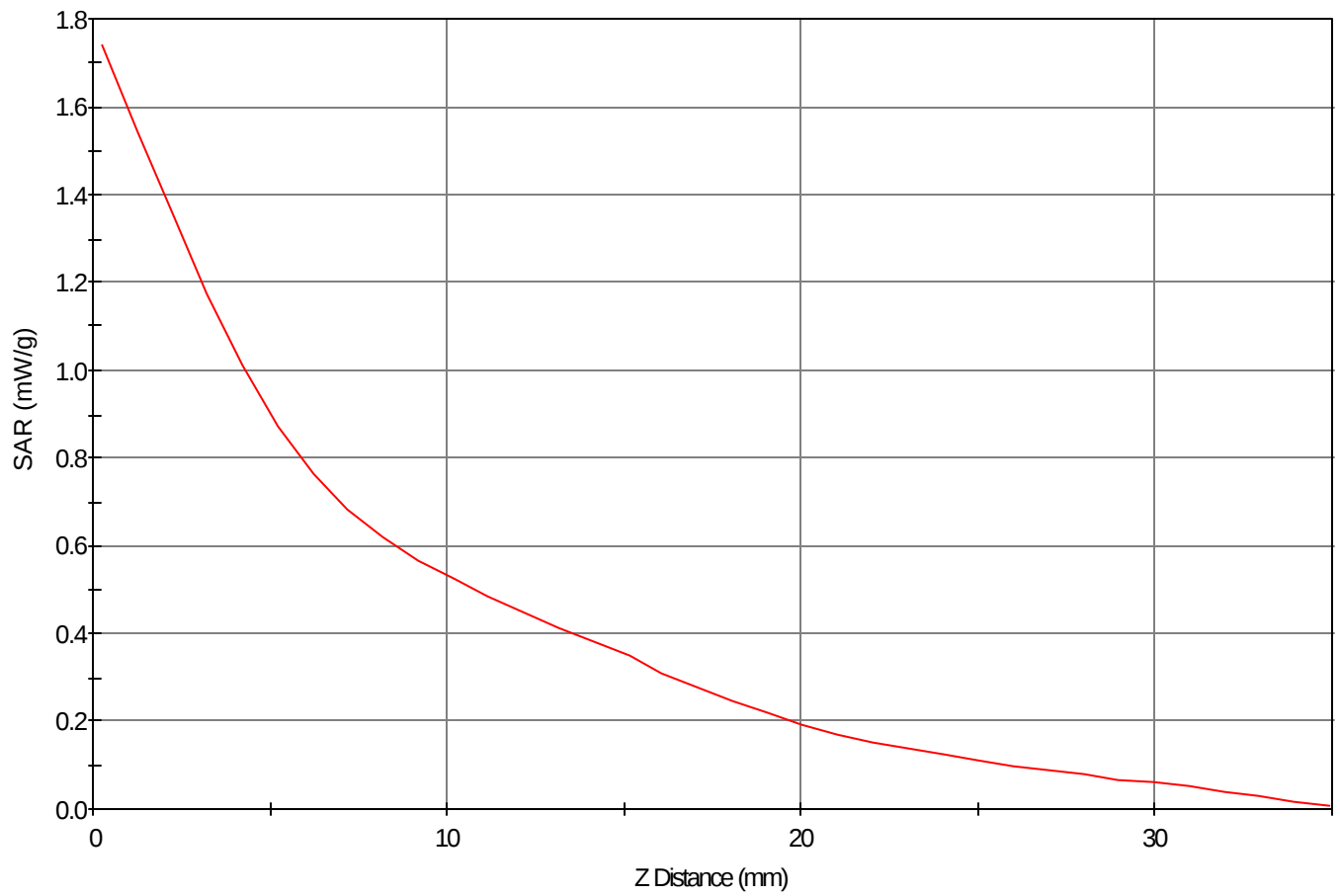
SAR - Z Axis at Hotspot x:-8.0 y:-21.0
