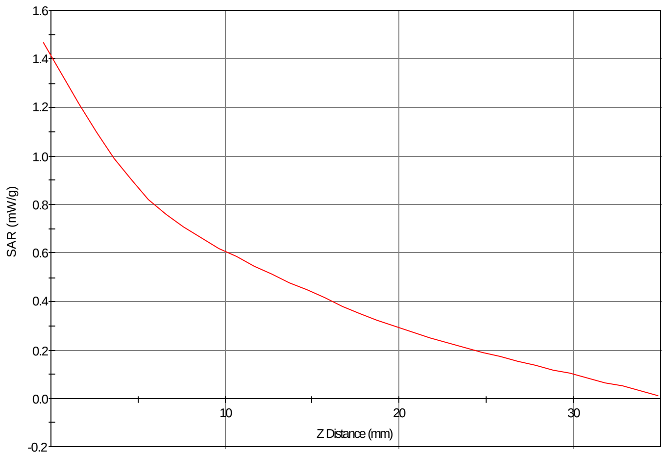
SAR - Z Axis at Hotspot x:67.0 y:11.0
