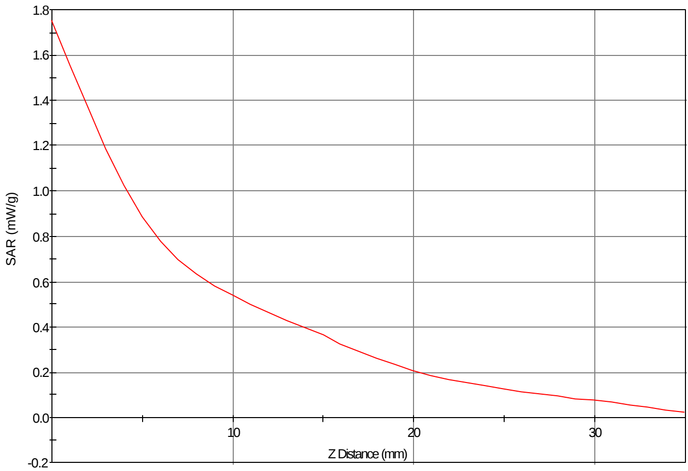
SAR - Z Axis at Hotspot x:56.0 y:9.0
