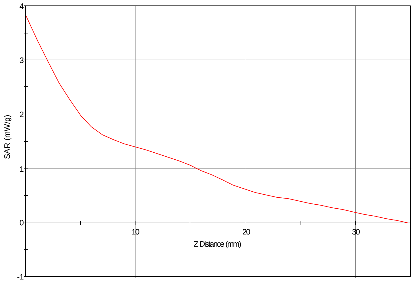
SAR - Z Axis at Hotspot x:57.0 y:18.0
