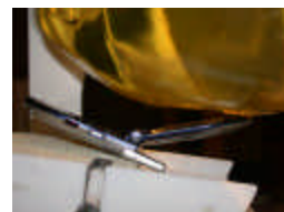
Figure A.8 Left Head SAR Test Setup -- Ear / 15° Tilt Position --
