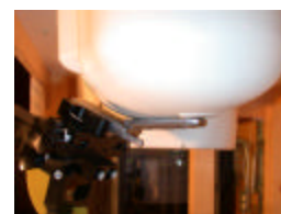
Figure 14.3 Left Head SAR Test Setup -- Cheek / Touch Position --
