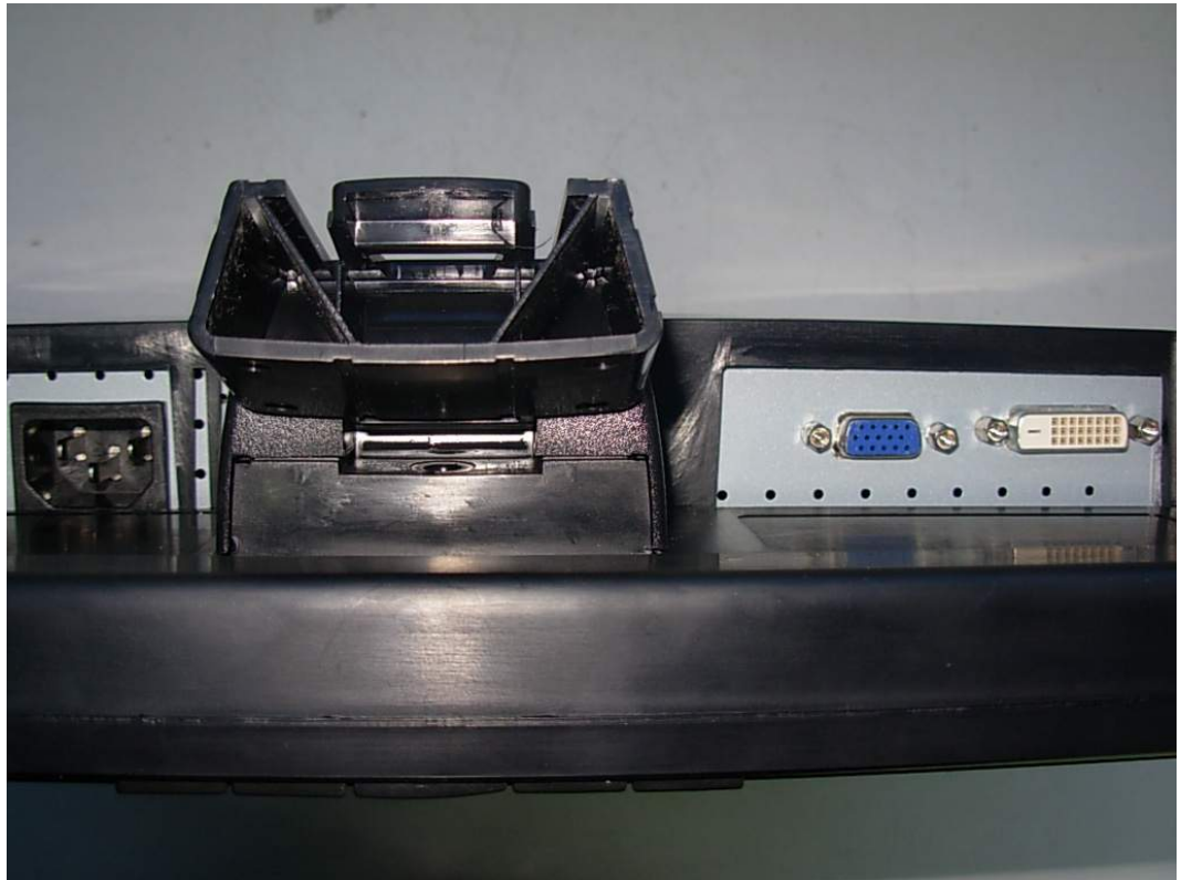
FIGURE 3 LCD MONITOR (M/N: L1742TT) PORTS VIEW
