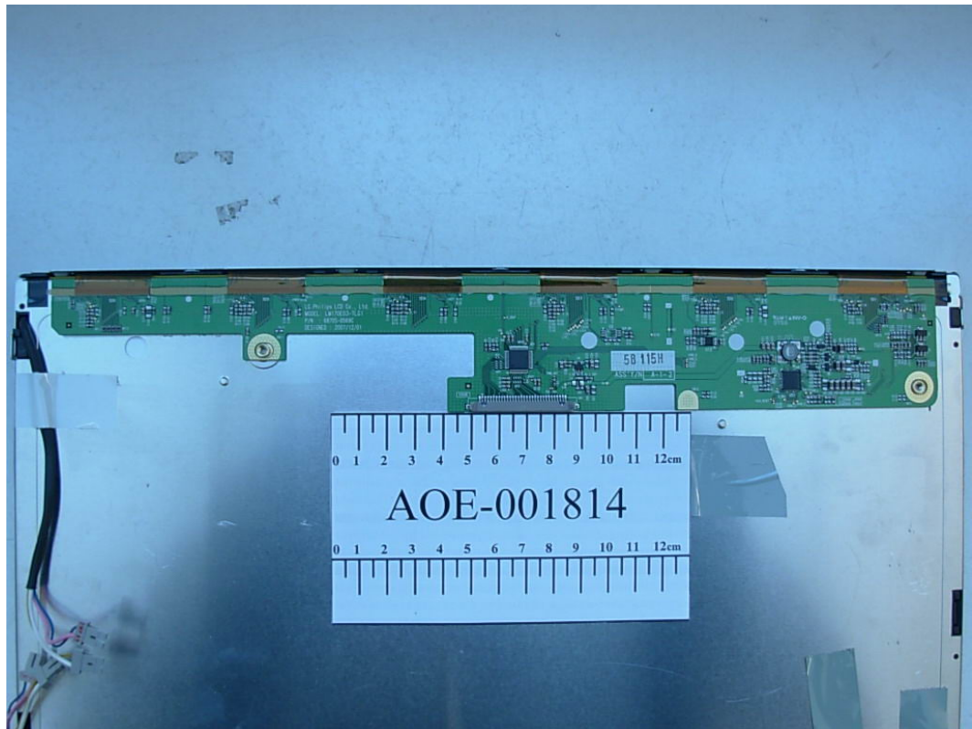
FIGURE 5 LCD MONITOR (M/N: L1742TT) LCD PANEL MAIN BOARD (COMPONENT SIDE)
