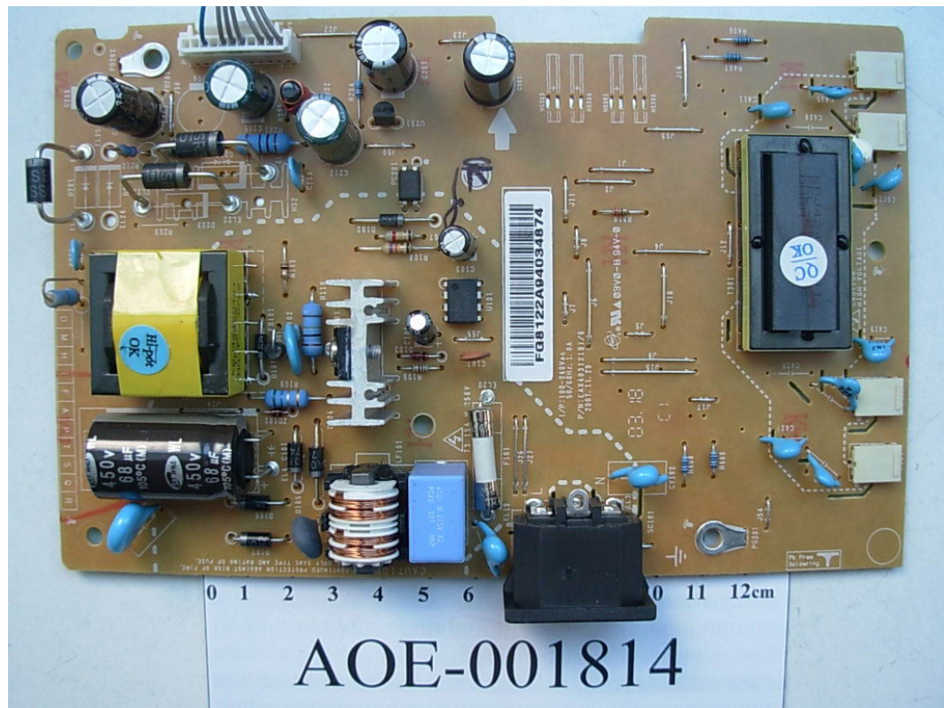
FIGURE 9 LCD MONITOR (M/N: L1742TT) POWER BOARD (COMPONENT SIDE)
