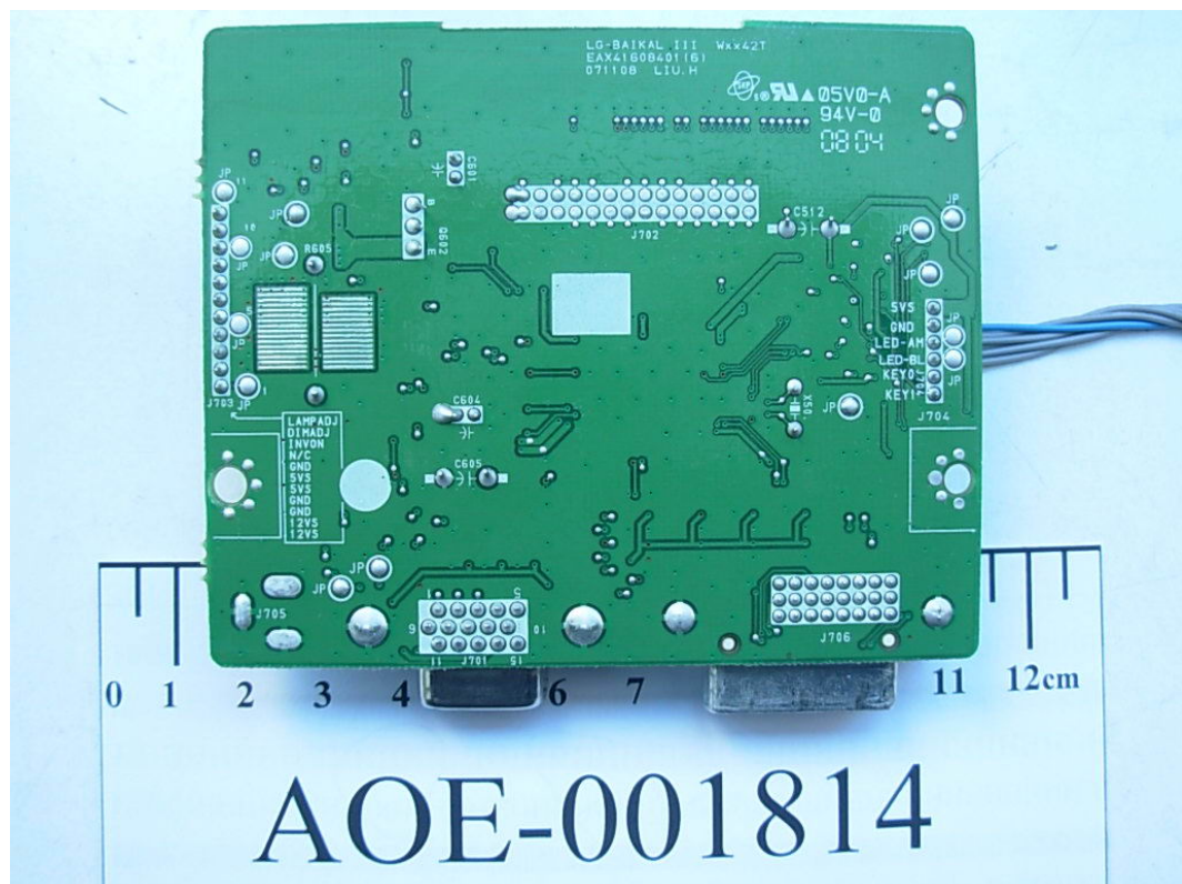
FIGURE 12 LCD MONITOR (M/N: L1742TT) MAIN BOARD (SOLDERED SIDE)
