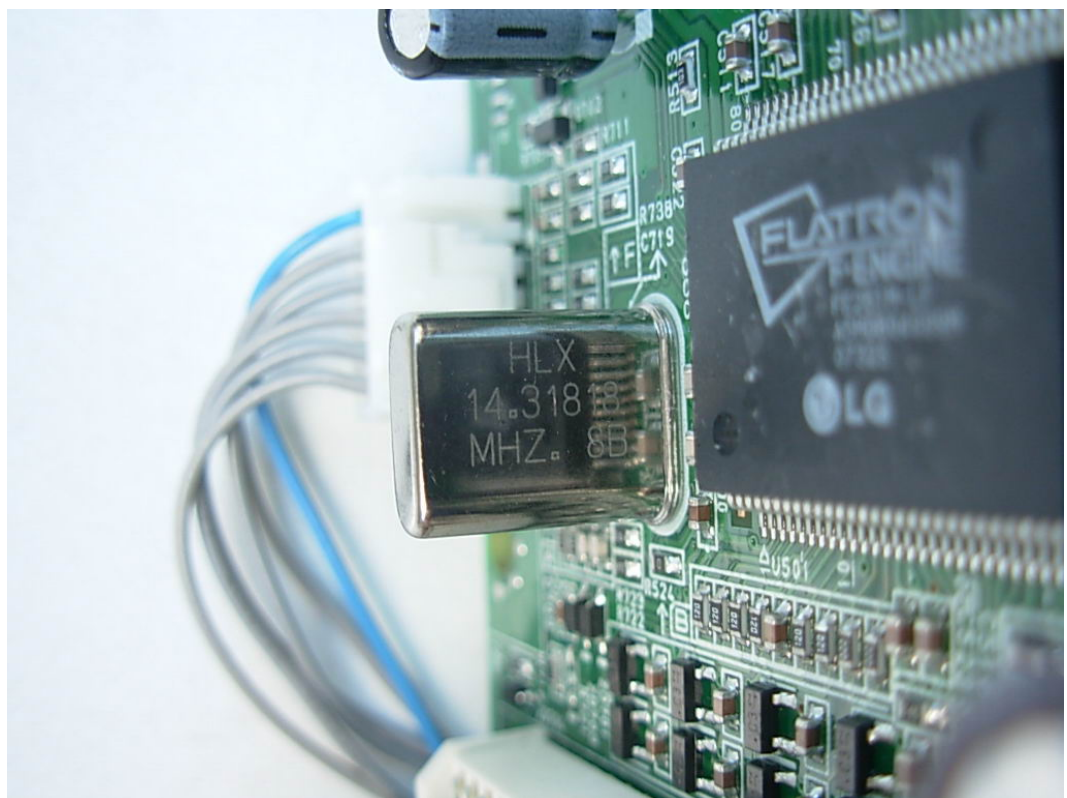
FIGURE 14 LCD MONITOR (M/N: L1742TT) CRYSTAL ON MAIN BOARD
