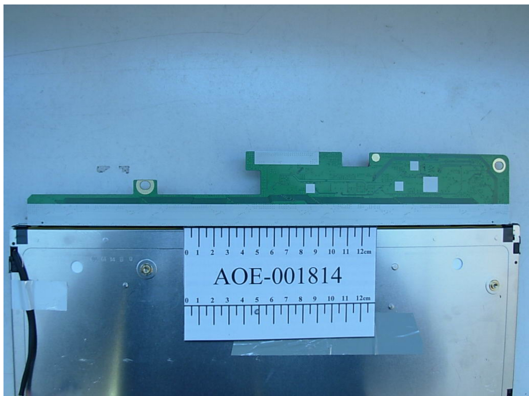
FIGURE 6 LCD MONITOR (M/N: L1742TT) LCD PANEL MAIN BOARD (SOLDERED SIDE)
