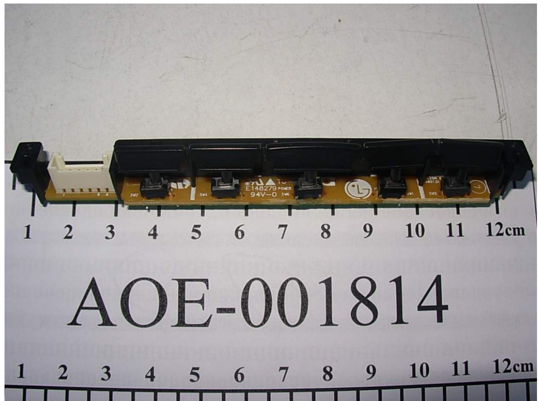
FIGURE 7 LCD MONITOR (M/N: L1742TT) BUTTON BOARD (COMPONENT SIDE)
