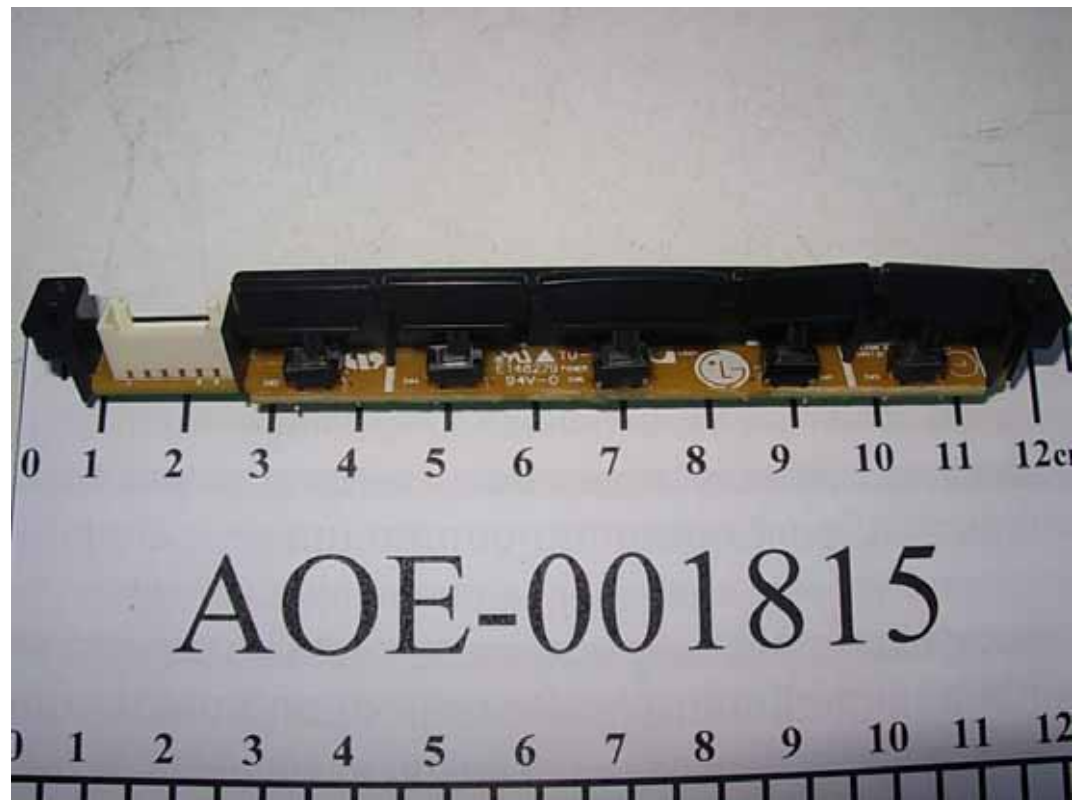
FIGURE 7 LCD MONITOR (M/N: L1742ST) BUTTON BOARD (COMPONENT SIDE)
