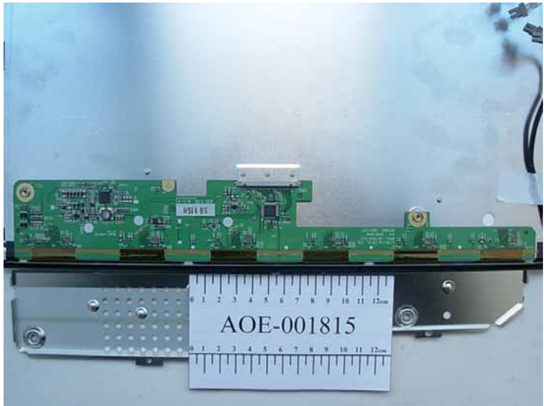
FIGURE 4 LCD MONITOR (M/N: L1742ST) LCD PANEL MAIN BOARD (COMPONENT SIDE)
