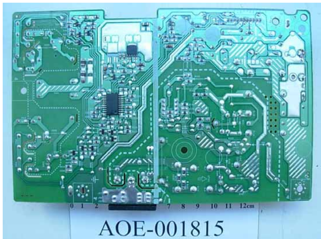
FIGURE 10 LCD MONITOR (M/N: L1742ST) POWER BOARD (SOLDERED SIDE)
