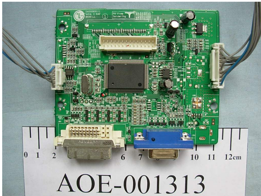
Figure 3 LCD MONITOR (M/N: L1753TS) MAIN BOARD (COMPONENT SIDE)
