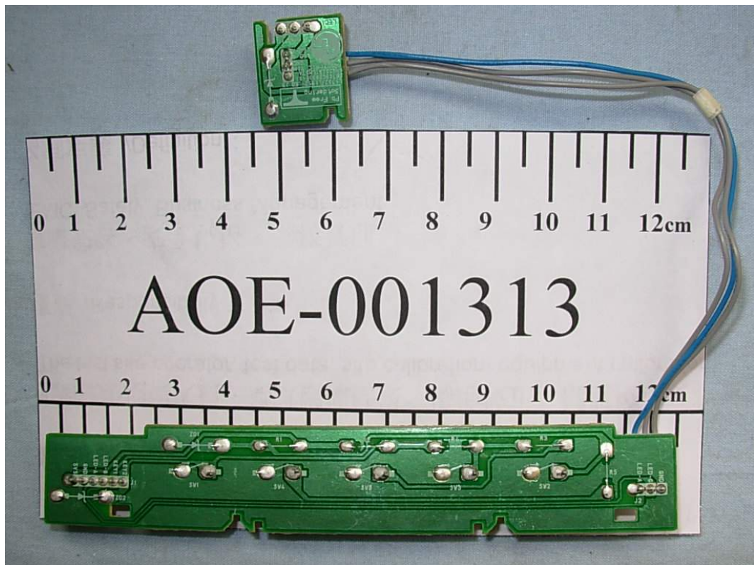
FIGURE 15 LCD MONITOR (M/N: L1753TS) SWITCH & LED BOARD (SOLDERED SIDE)
