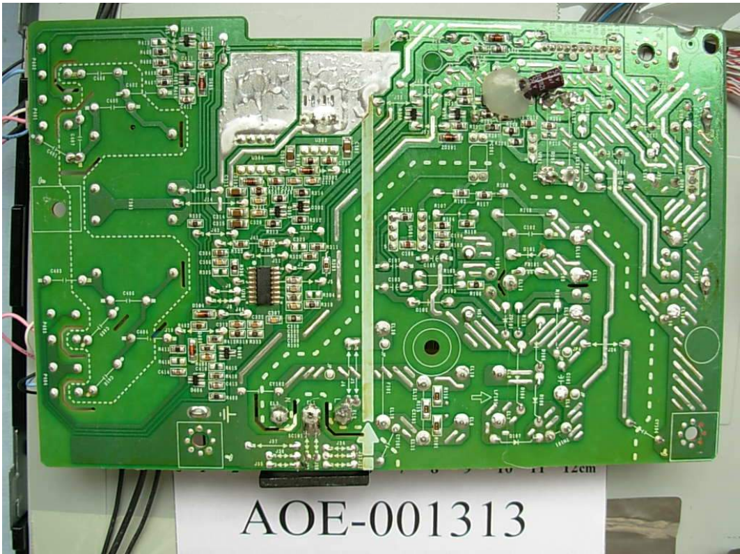
FIGURE 8 LCD MONITOR (M/N: L1753TS) POWER BOARD (SOLDERED SIDE)
