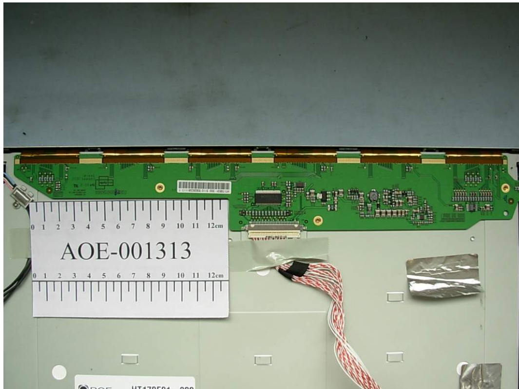
FIGURE 11 LCD MONITOR (M/N: L1753TS) LCD PANEL MAIN BOARD (COMPONENT SIDE)
