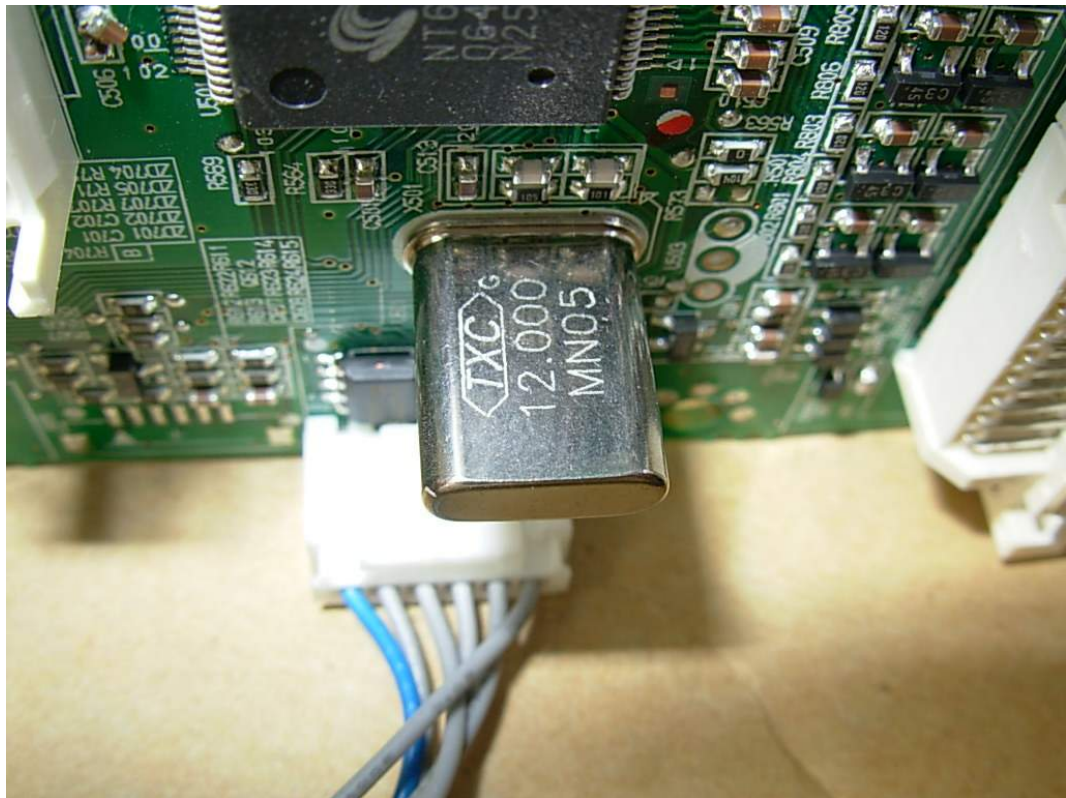
Figure 5 LCD MONITOR (M/N: L1753TS) CRYSTAL ON MAIN BOARD
