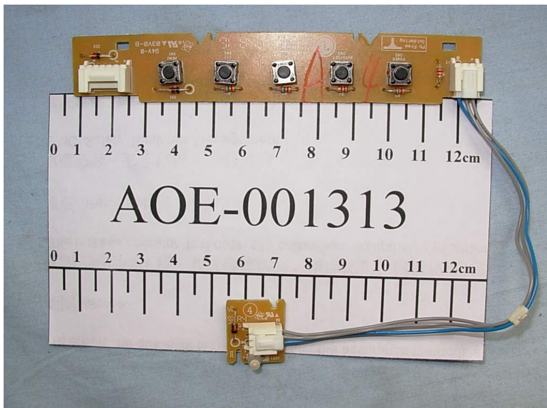
Figure 14 LCD MONITOR (M/N: L1753TS) SWITCH & LED BOARD (COMPONENT SIDE)
