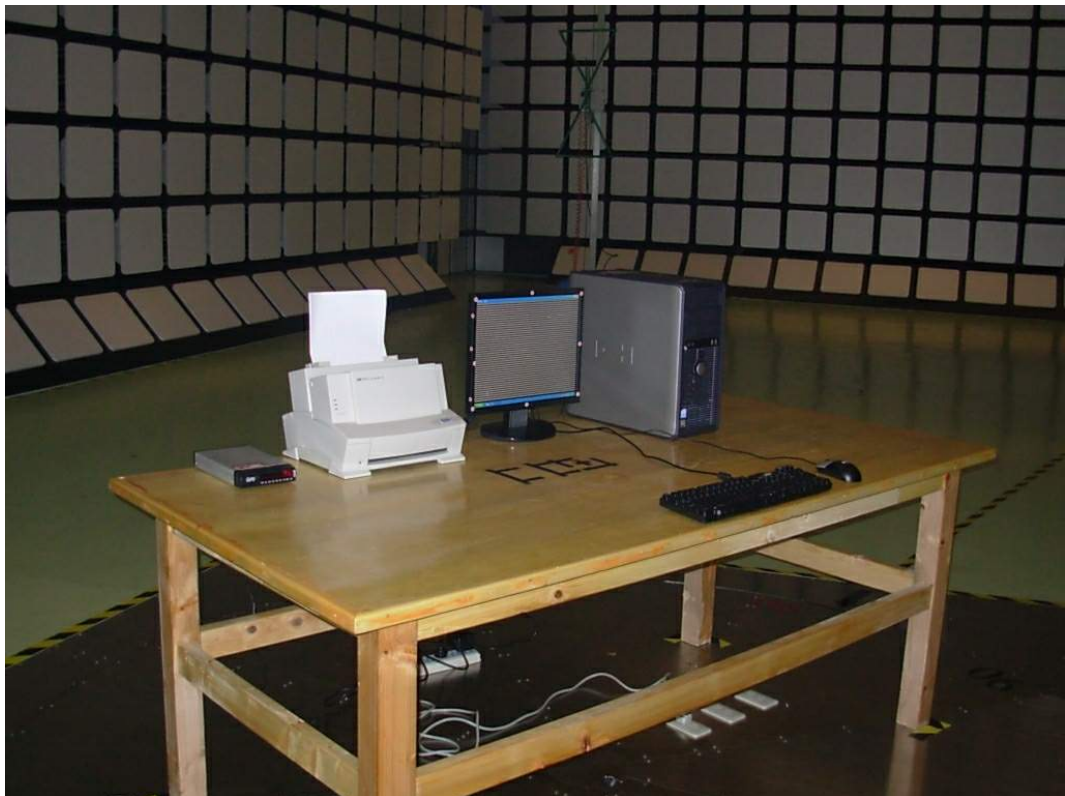
SETUP WITH MAXIMUM DETECTED EMISSION AT VERTICAL POLARIZATION (VGA 1024*768@75Hz)
