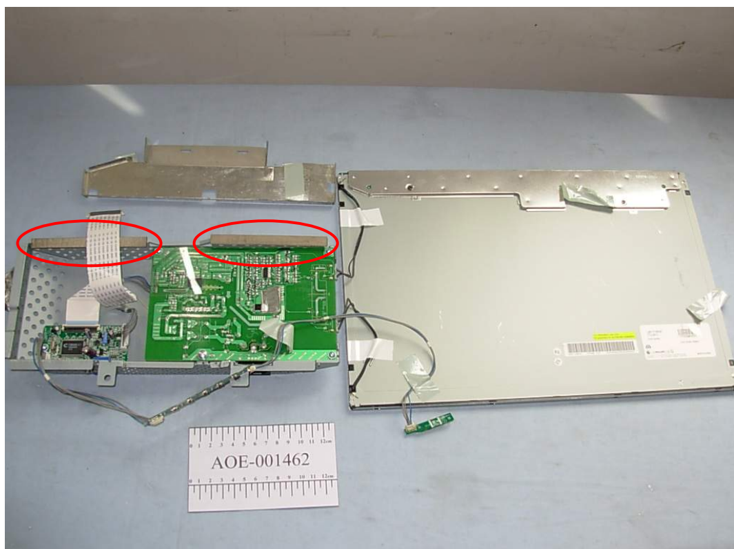
FIGURE 2 LCD MONITOR (M/N: L177WSBS) BOARDS REMOVED
