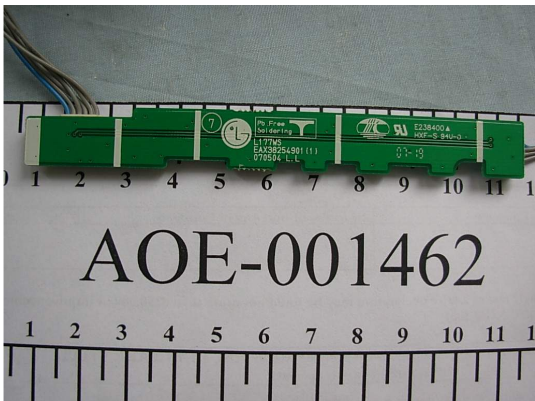
FIGURE 6 LCD MONITOR (M/N: L177WSBS) BUTTON BOARD BACK
