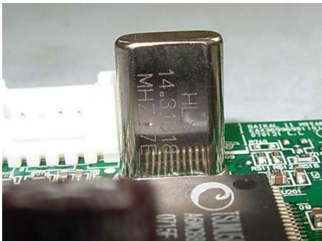
FIGURE 10 LCD MONITOR (M/N: L177WSBS) CRYSTAL ON MAIN BOARD
