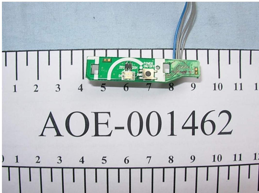
FIGURE 4 LCD MONITOR (M/N: L177WSBS) LED BOARD BACK
