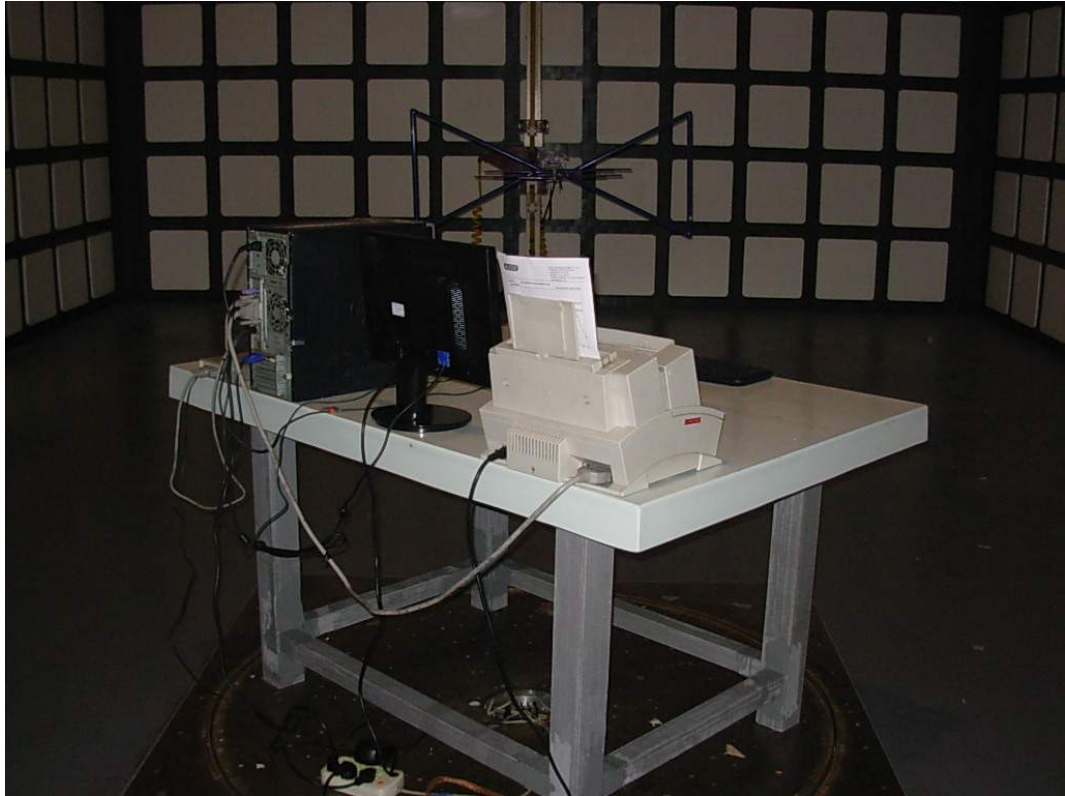
SETUP WITH MAXIMUM DETECTED EMISSION AT HORIZONTAL POLARIZATION (VGA 1440*900@75Hz, LOW FREQUENCY)
