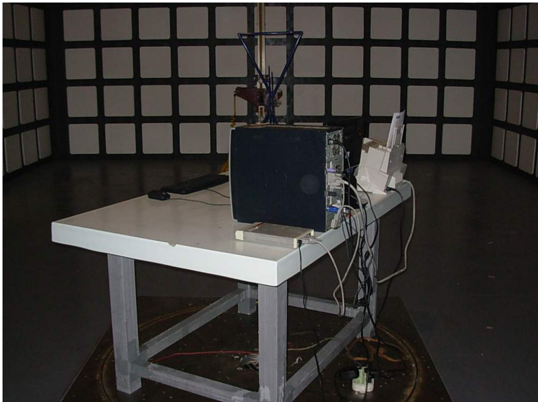
SETUP WITH MAXIMUM DETECTED EMISSION AT VERTICAL POLARIZATION (VGA 1440*900@75Hz, LOW FREQUENCY)
