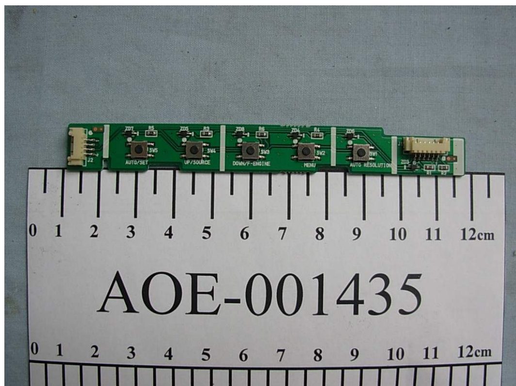
FIGURE 12 LCD MONITOR (M/N: L177WSS) BUTTON BOARD FRONT
