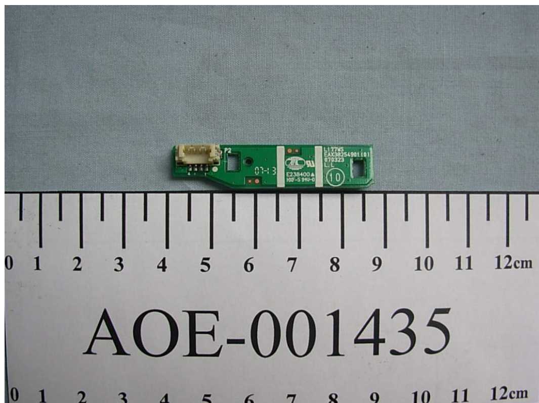
FIGURE 10 LCD MONITOR (M/N: L177WSS) LED BOARD FRONT
