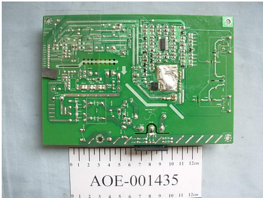
FIGURE 5 LCD MONITOR (M/N: L177WSS) POWER BOARD (SOLDERED SIDE)
