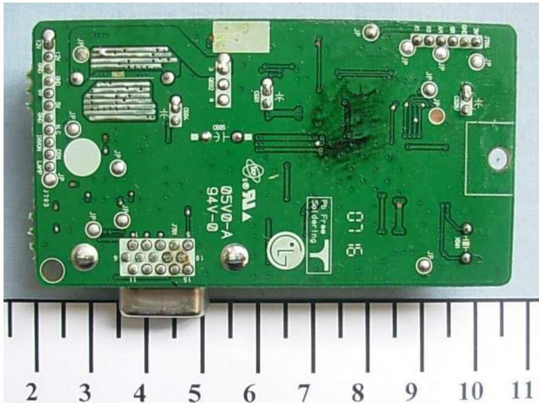
FIGURE 7 LCD MONITOR (M/N: L177WSS) MAIN BOARD (SOLDERED SIDE)
