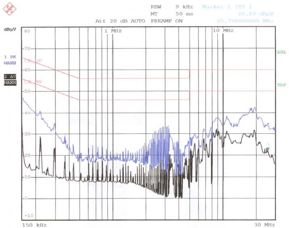
< Neutral line >
