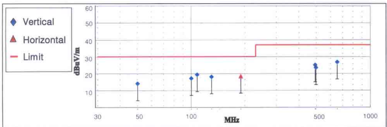
< Fig 5. Radiated emission result-Digital >
