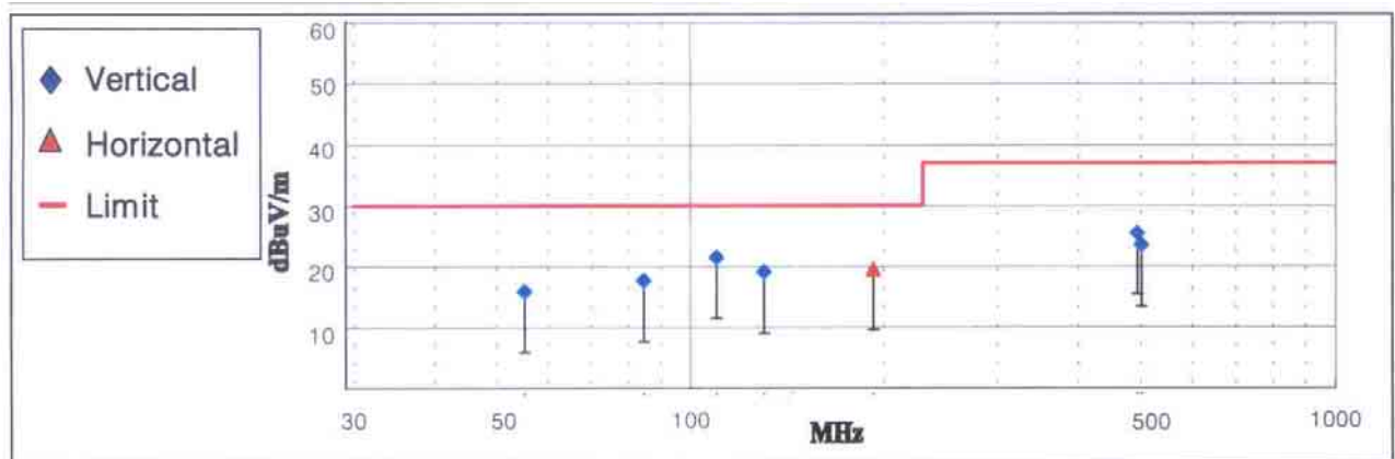
< Fig 4. Radiated emission result-Analog >
