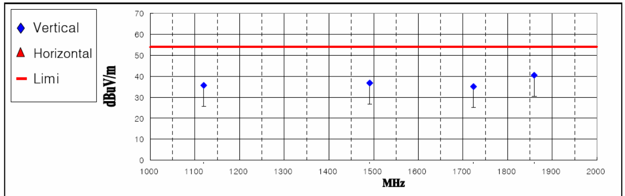
< Fig 6. Radiated emission result (1000MHz ~ 2000MHz)>
