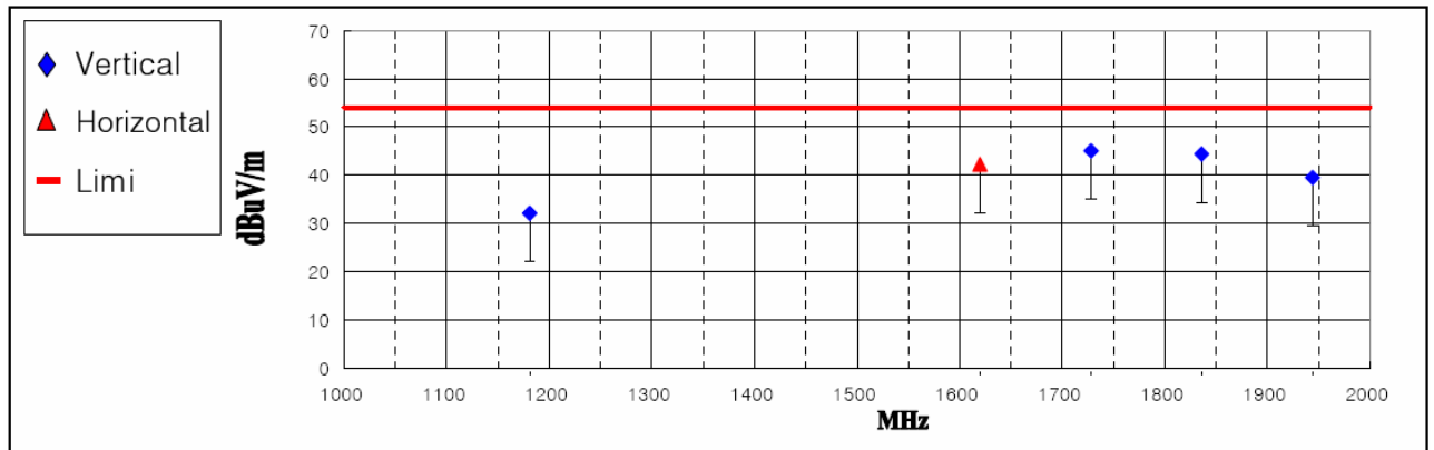
< Fig 7. Radiated emission result (1000MHz ~ 2000MHz)>
