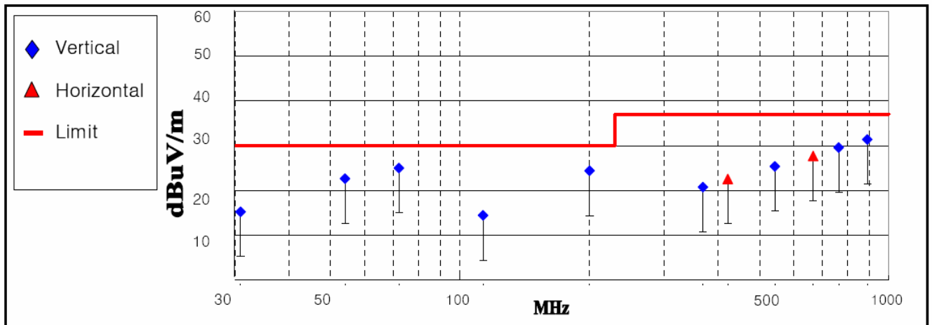
< Fig 4. Radiated emission result (30MHz ~ 1000MHz)>
