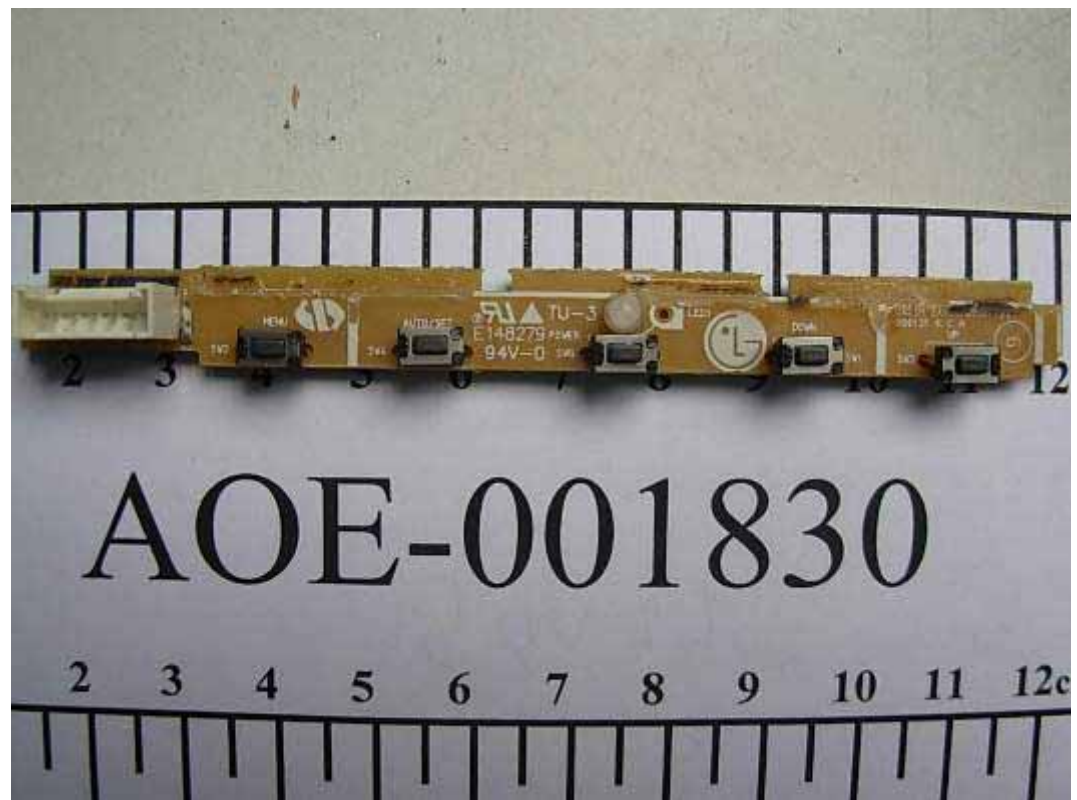
FIGURE 3 LCD MONITOR (M/N: L1942TT) BUTTON BOARD (COMPONENT SIDE)
