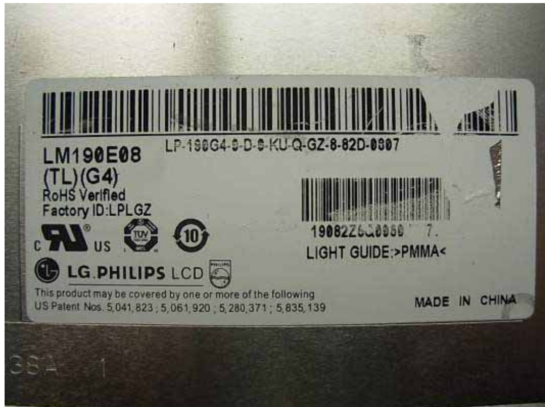
FIGURE 11 LCD MONITOR (M/N: L1942TT) LCD PANEL LABEL #1
