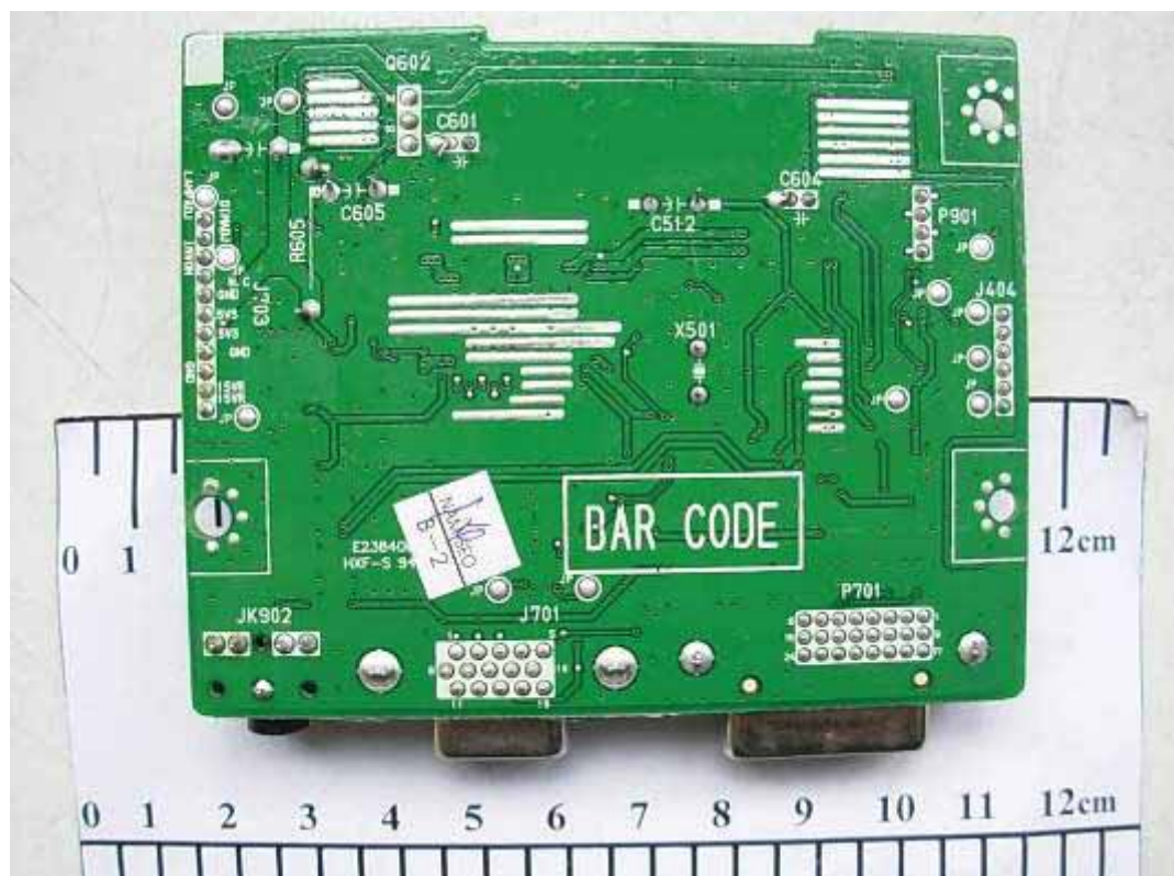
FIGURE 8 LCD MONITOR (M/N: L1942PKU) MAIN BOARD (SOLDERED SIDE)
