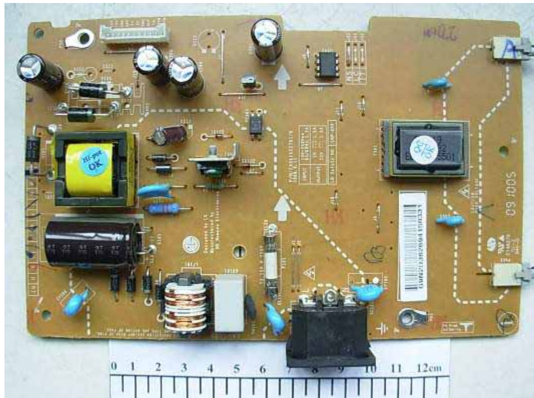
FIGURE 10 LCD MONITOR (M/N: L1942PKU) POWER BOARD (COMPONENT SIDE)
