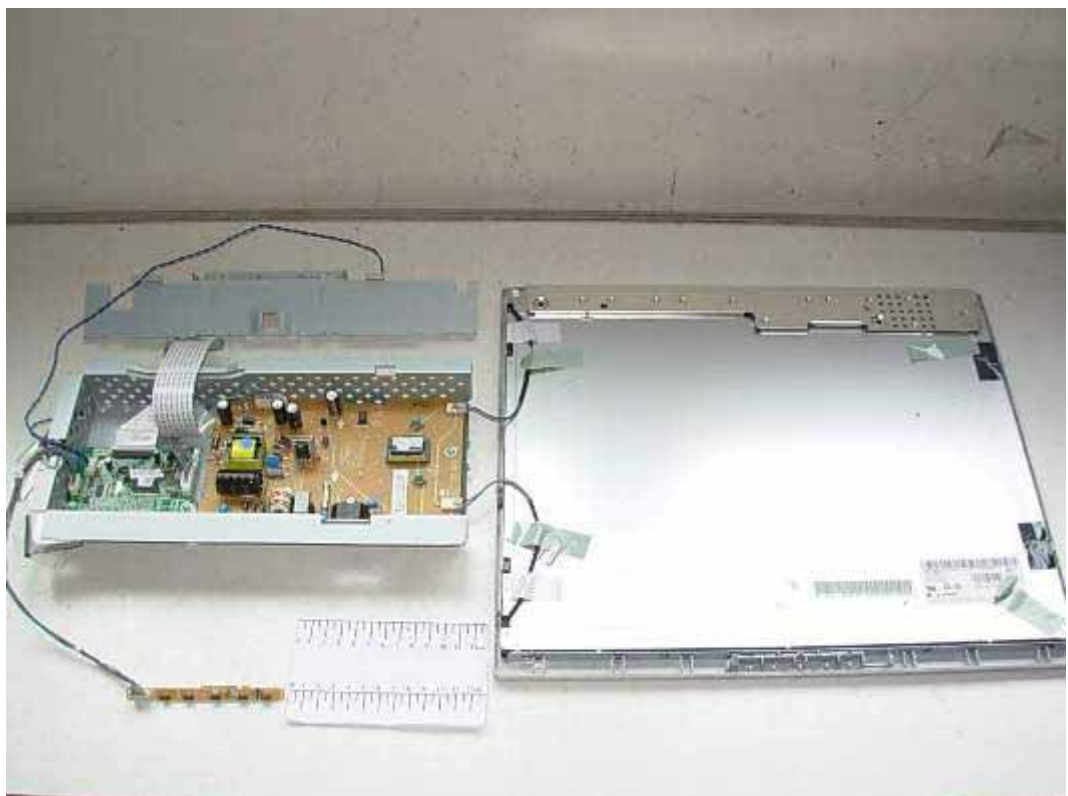
FIGURE 4 LCD MONITOR (M/N: L1942PKU) BOARDS REMOVED
