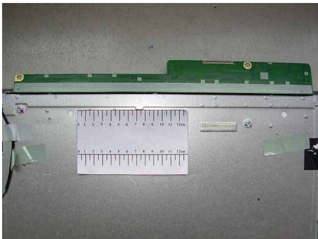
FIGURE 14 LCD MONITOR (M/N: L1942PKU) LCD PANEL BOARD (SOLDERED SIDE)
