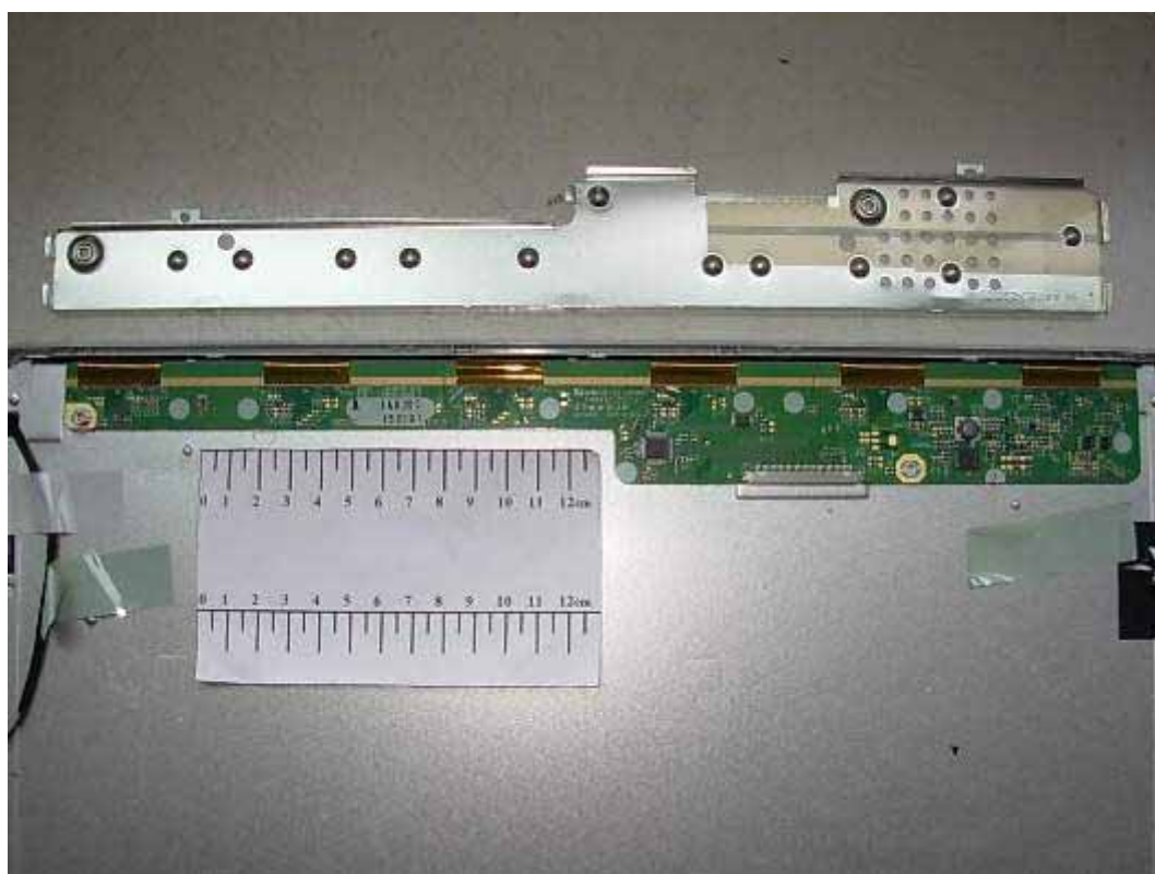
FIGURE 13 LCD MONITOR (M/N: L1942PKU) LCD PANEL BOARD (COMPONENT SIDE)
