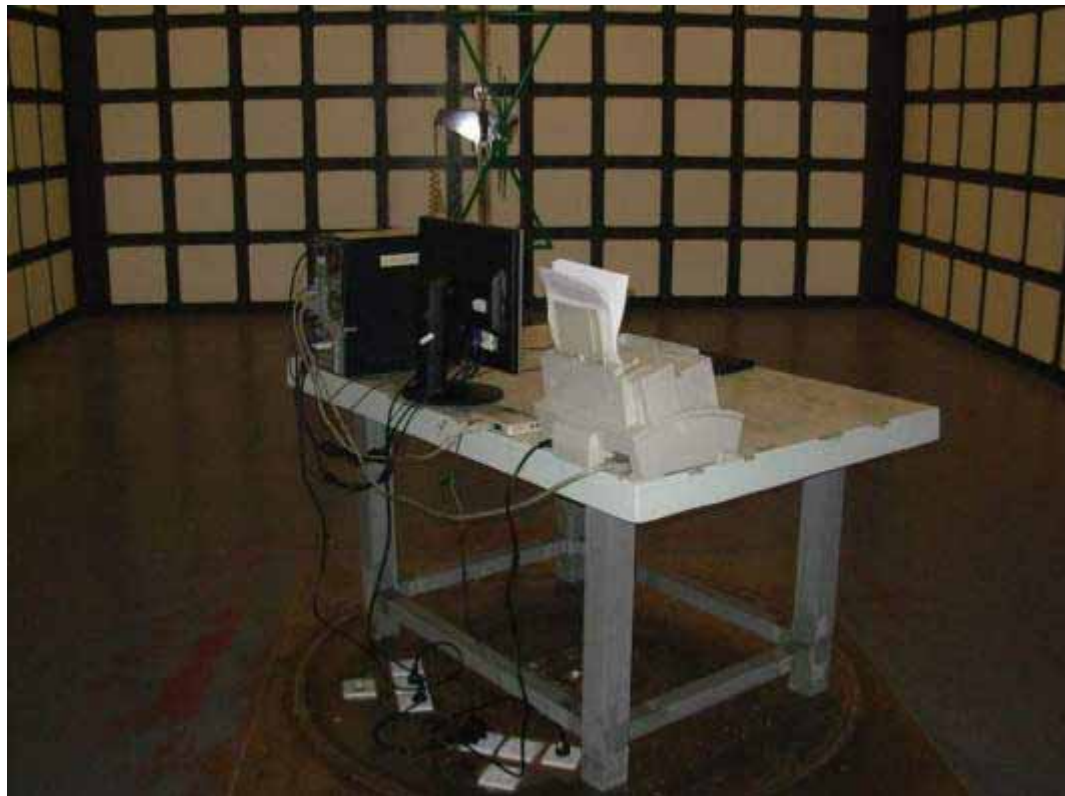
SETUP WITH MAXIMUM DETECTED EMISSION AT VERTICAL POLARIZATION (TEST MODE: DVI 1280*1024@60Hz)
