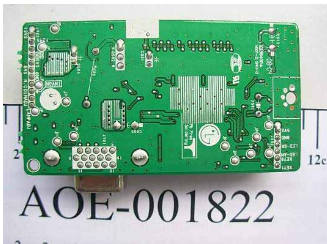
FIGURE 6 LCD MONITOR (M/N: L1942ST) MAIN BOARD (SOLDERED SIDE)
