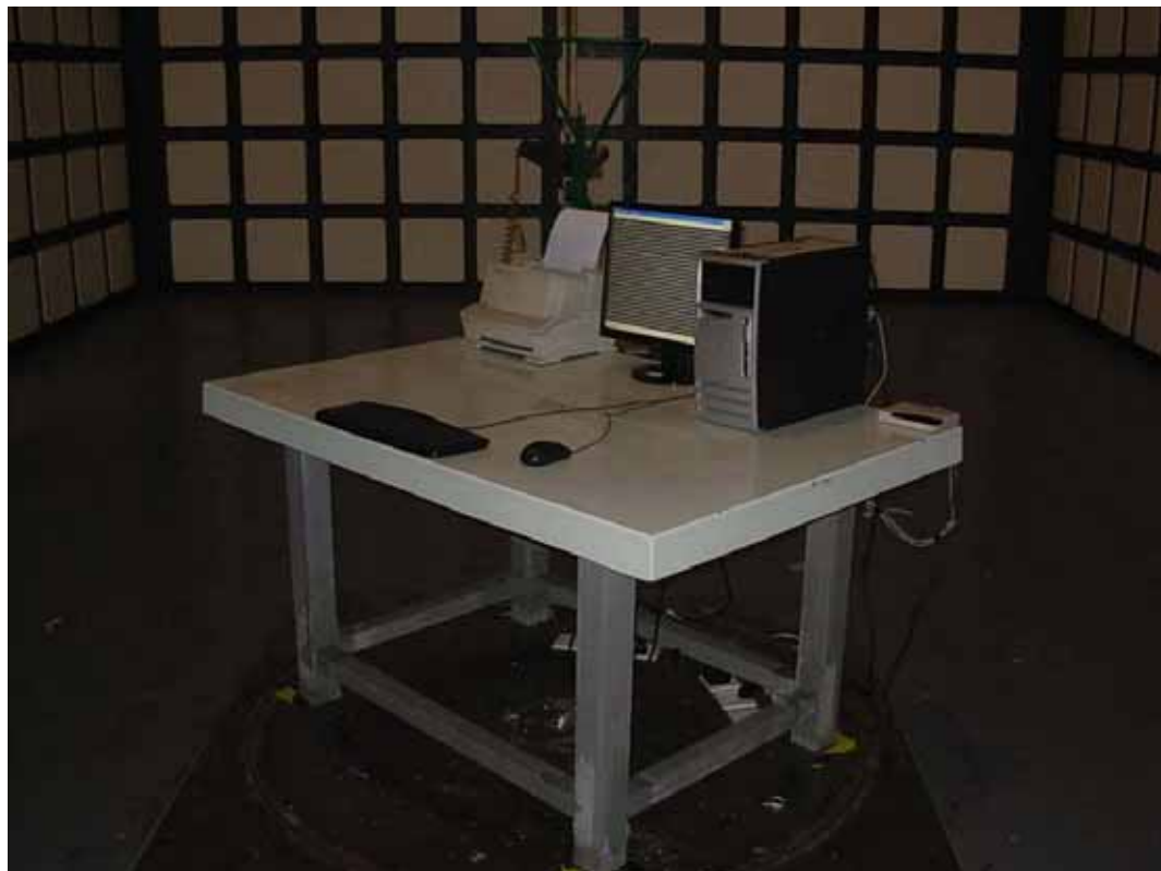
SETUP WITH MAXIMUM DETECTED EMISSION AT VERTICAL POLARIZATION (VGA 640*480@60Hz)
