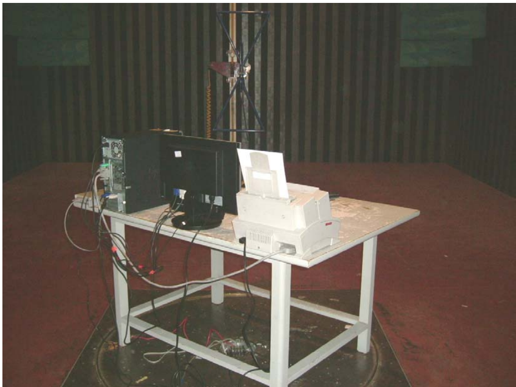
SETUP WITH MAXIMUM DETECTED EMISSION AT VERTICAL POLARIZATION (DVI 1280*1024@75Hz)
