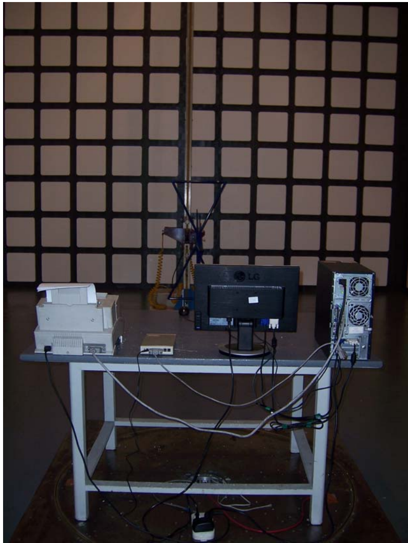
BACK VIEW OF RADIATED EMISSION TEST (LOW FREQUENCY)
