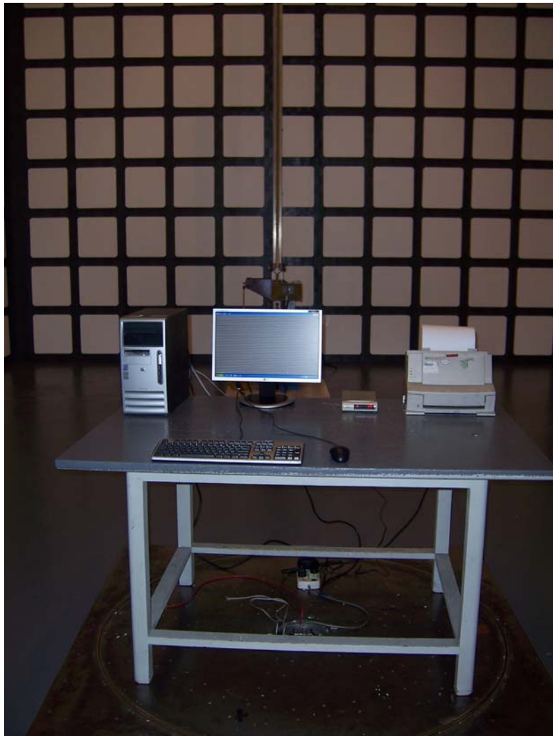
FRONT VIEW OF RADIATED EMISSION TEST (HIGH FREQUENCY)
