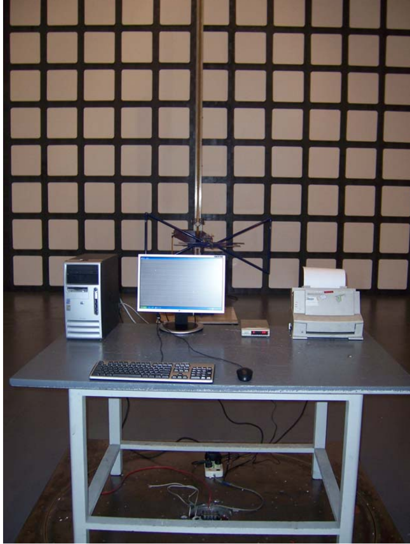
FRONT VIEW OF RADIATED EMISSION TEST (LOW FREQUENCY)
