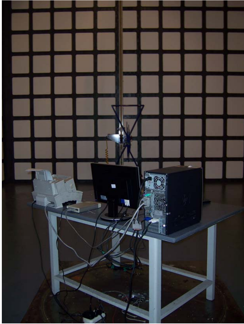
SETUP WITH MAXIMUM DETECTED EMISSION AT VERTICAL POLARIZATION (DVI 1280*1024@75Hz)
