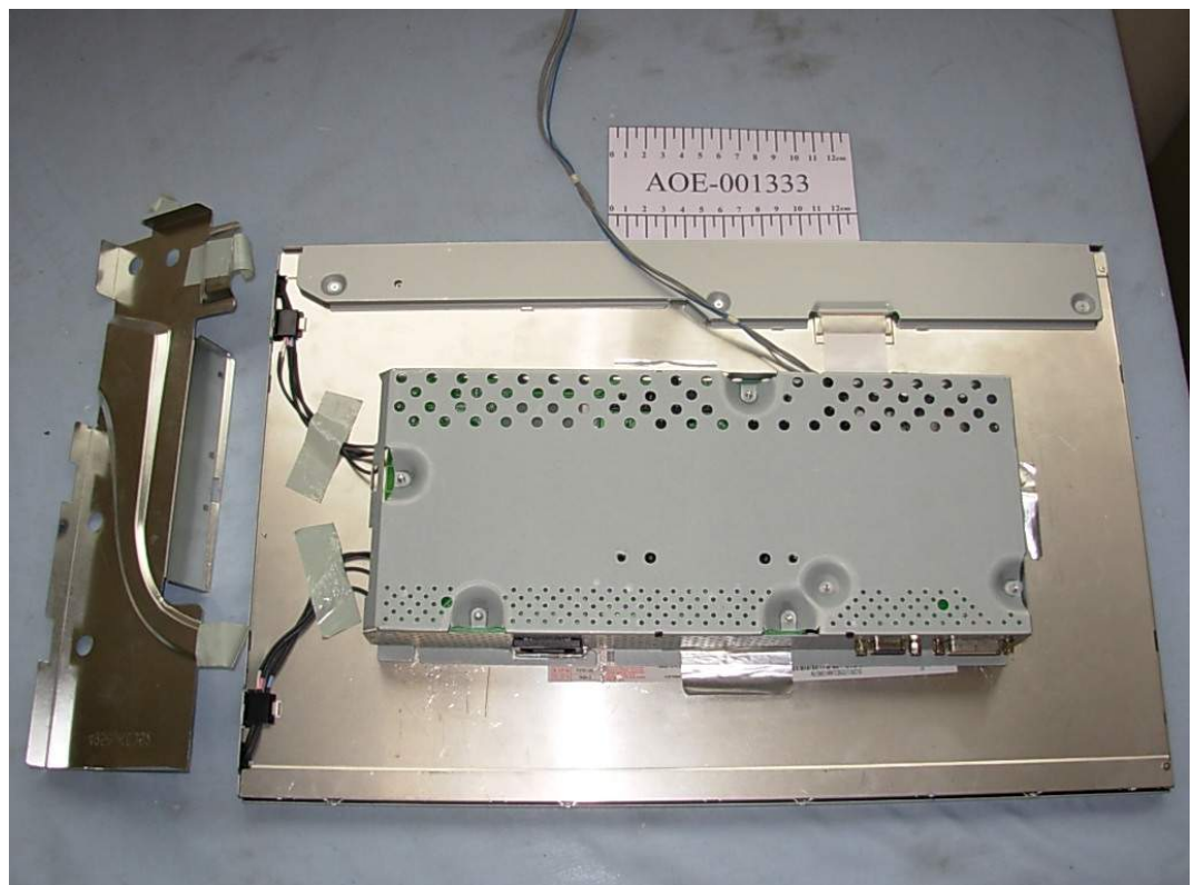
FIGURE 2 LCD MONITOR (M/N: L194WTS) SHIELDED COVER REMOVED
