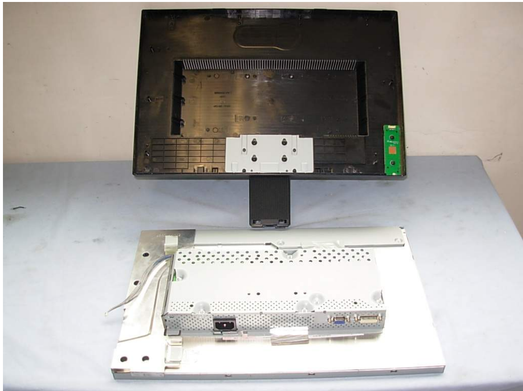
FIGURE 1 LCD MONITOR (M/N: L194WTS) COVER REMOVED
