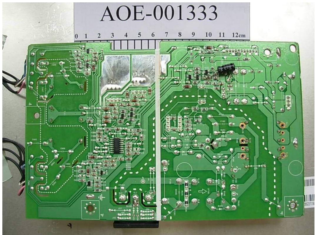
FIGURE 5 LCD MONITOR (M/N: L194WTS) POWER BOARD (SOLDERED SIDE)
