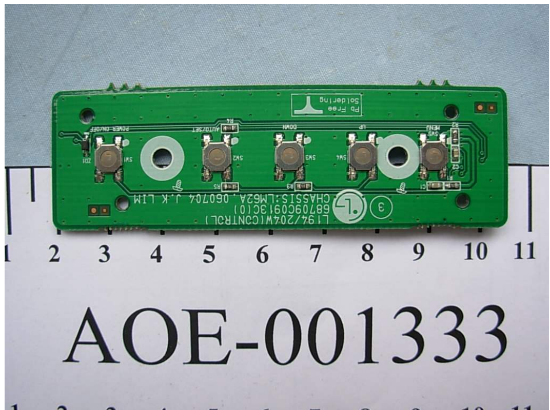
FIGURE 17 LCD MONITOR (M/N: L194WTS) SWITCH BOARD FRONT
