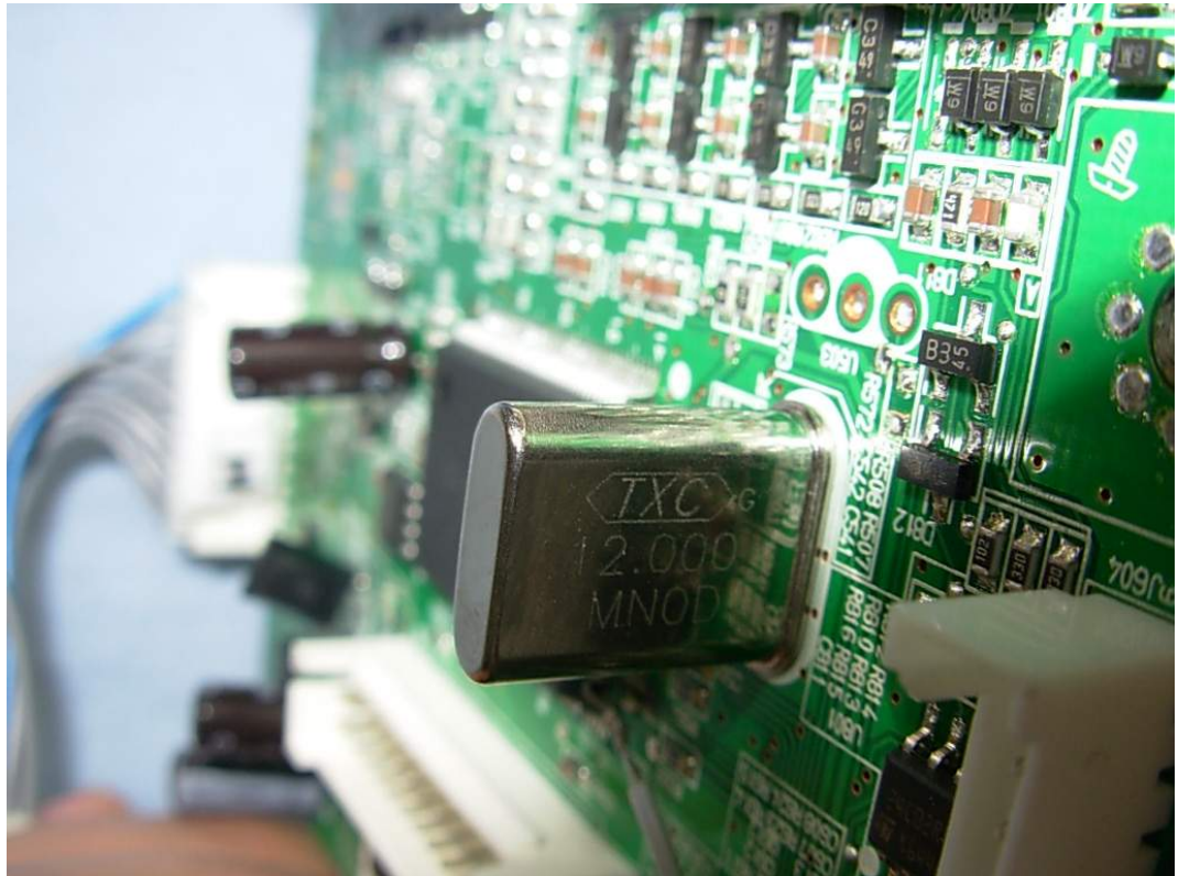
FIGURE 10 LCD MONITOR (M/N: L194WTS) LCD PANEL MAIN BOARD SHIELDED COVER REMOVED
