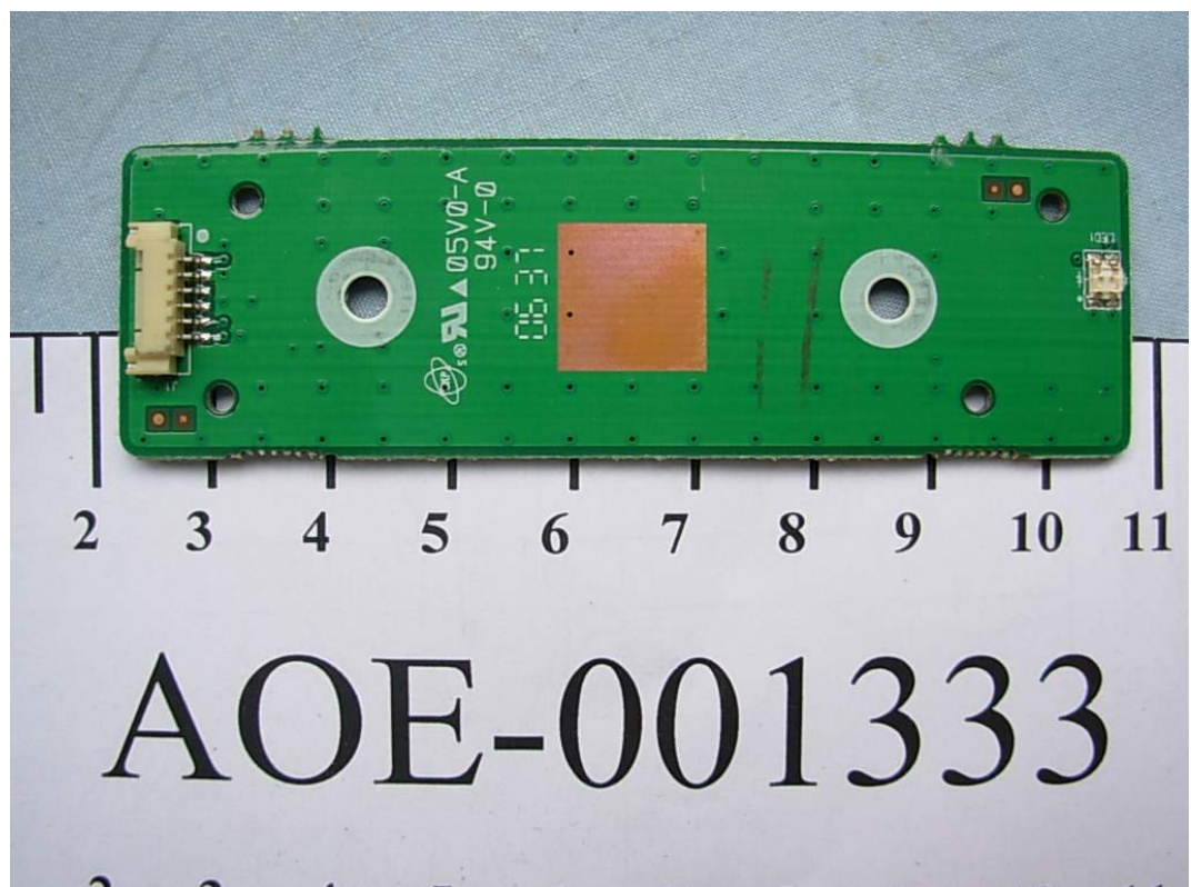
FIGURE 18 LCD MONITOR (M/N: L194WTS) SWITCH BOARD BACK
