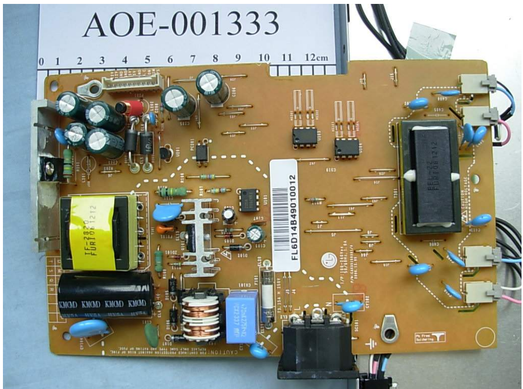
FIGURE 4 LCD MONITOR (M/N: L194WTS) POWER BOARD (COMPONENT SIDE)
