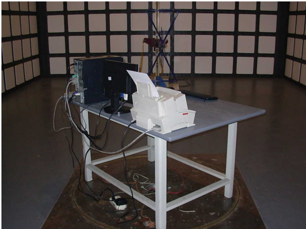
SETUP WITH MAXIMUM DETECTED EMISSION AT VERTICAL POLARIZATION (VGA 1440*900@60Hz)
