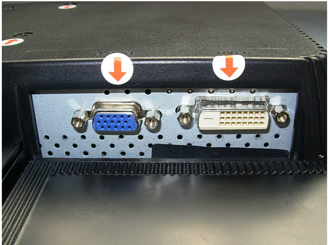
FIGURE 5 LCD MONITOR (M/N: L1953TS) PORTS
