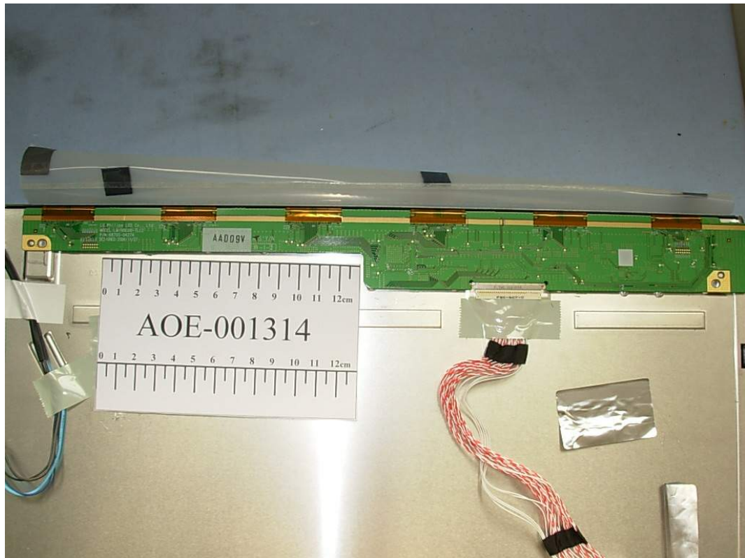
FIGURE 14 LCD MONITOR (M/N: L1953TS) LCD PANEL MAIN BOARD (SOLDERED SIDE)
