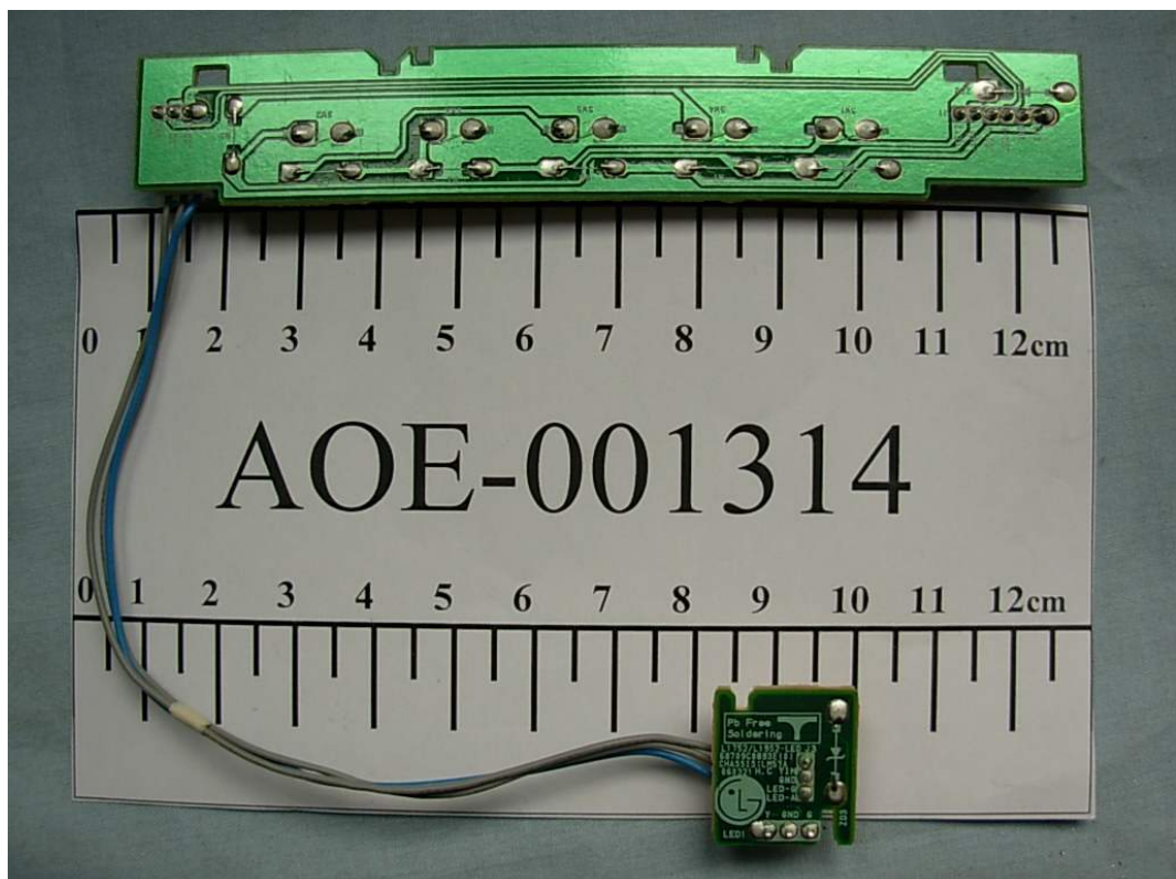
FIGURE 17 LCD MONITOR (M/N: L1953TS) SWITCH & LED BOARD (SOLDERED SIDE)
