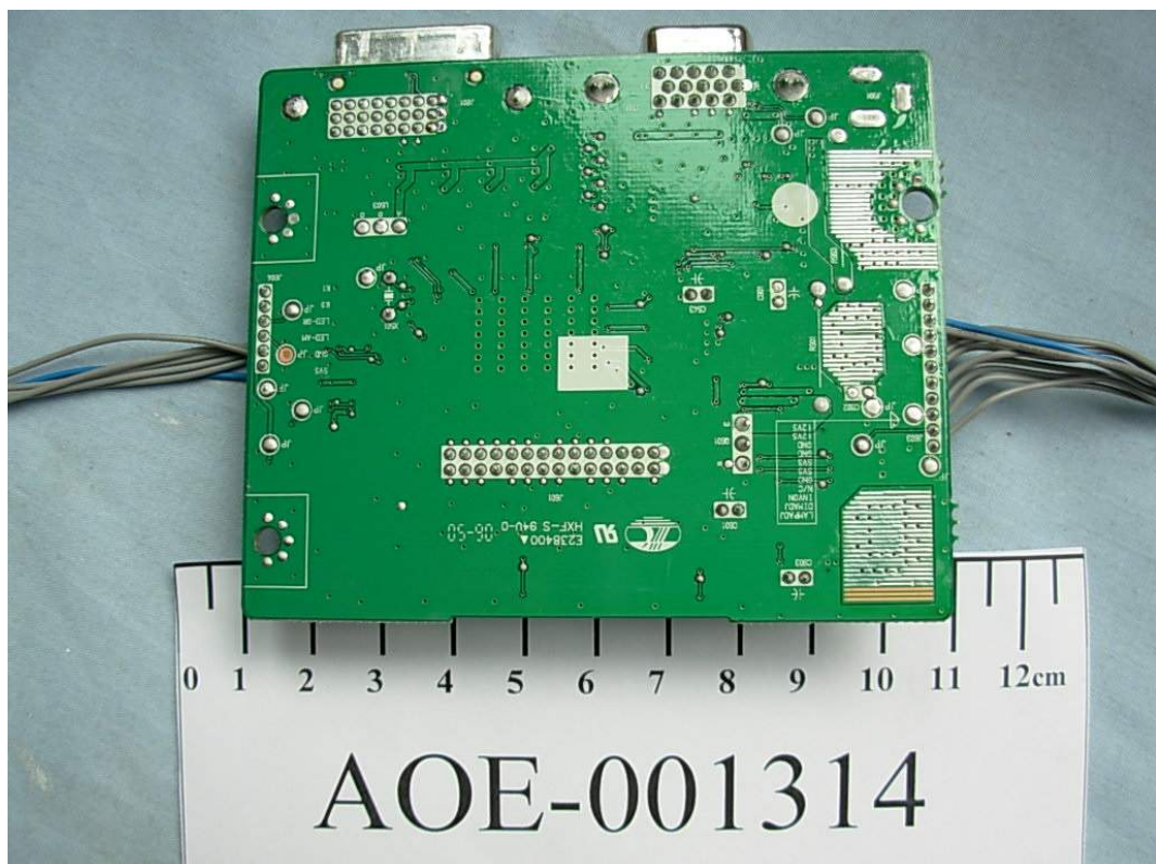
FIGURE 5 LCD MONITOR (M/N: L1953TS) MAIN BOARD (SOLDERED SIDE)
