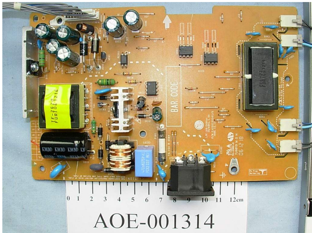
FIGURE 8 LCD MONITOR (M/N: L1953TS) POWER BOARD (COMPONENT SIDE)
