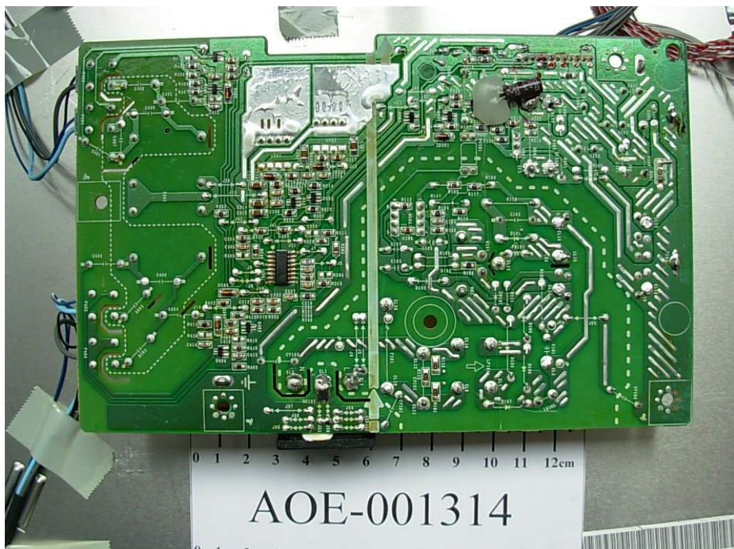
FIGURE 9 LCD MONITOR (M/N: L1953TS) POWER BOARD (SOLDERED SIDE)
