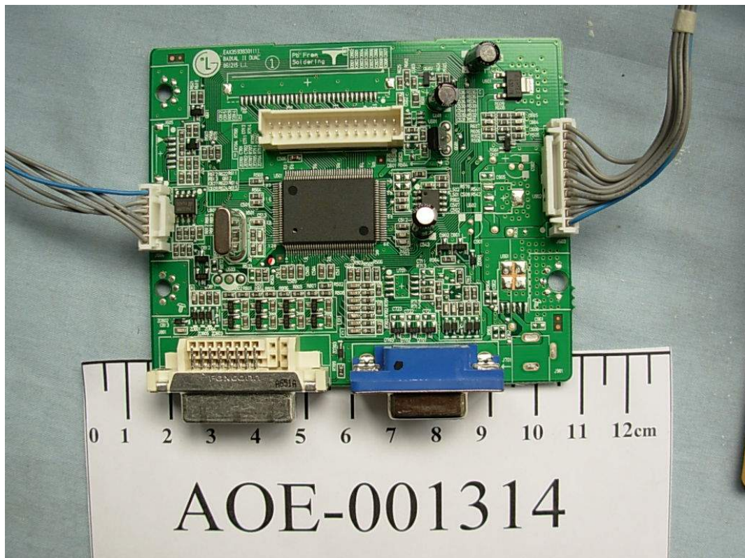
FIGURE 4 LCD MONITOR (M/N: L1953TS) MAIN BOARD (COMPONENT SIDE)
