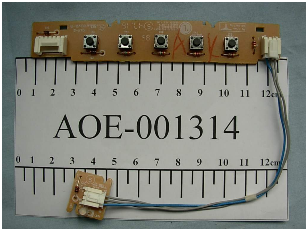
FIGURE 16 LCD MONITOR (M/N: L1953TS) SWITCH & LED BOARD (COMPONENT SIDE)
